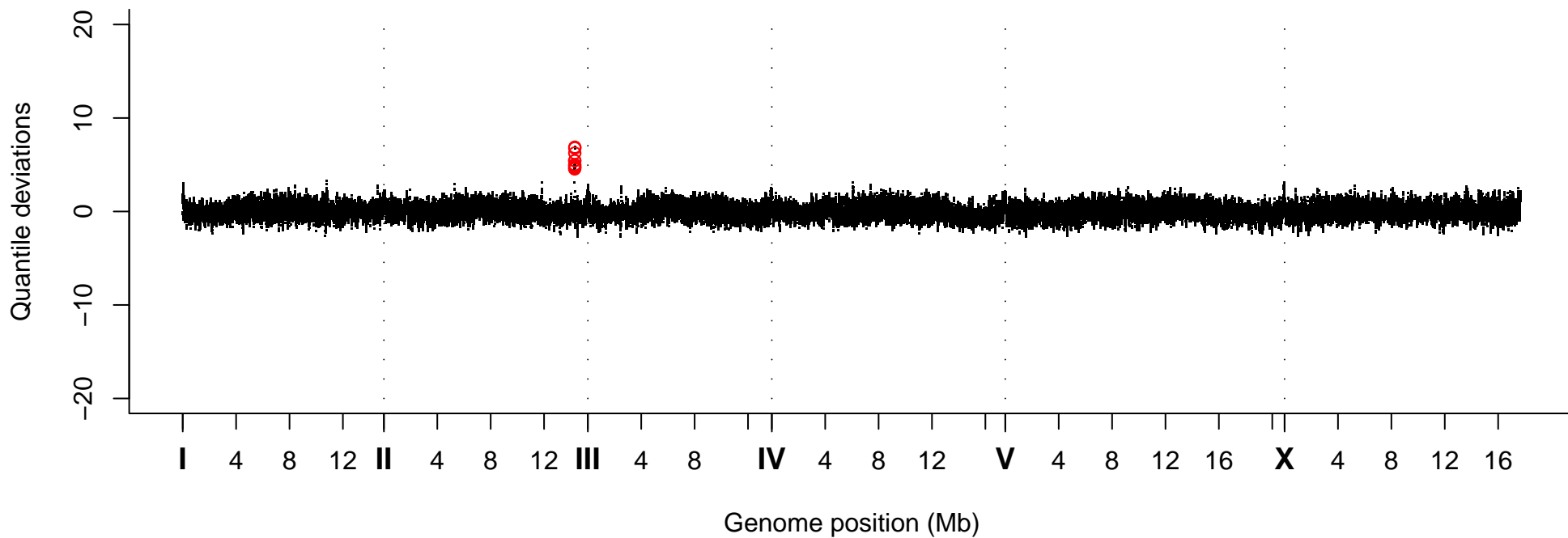
Quantile Deviations, Strain VC40077
