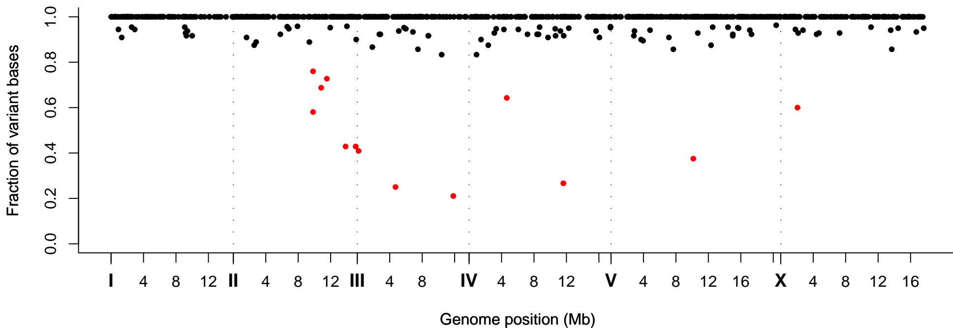
Fraction of Variant Bases at Position, Strain VC40077
