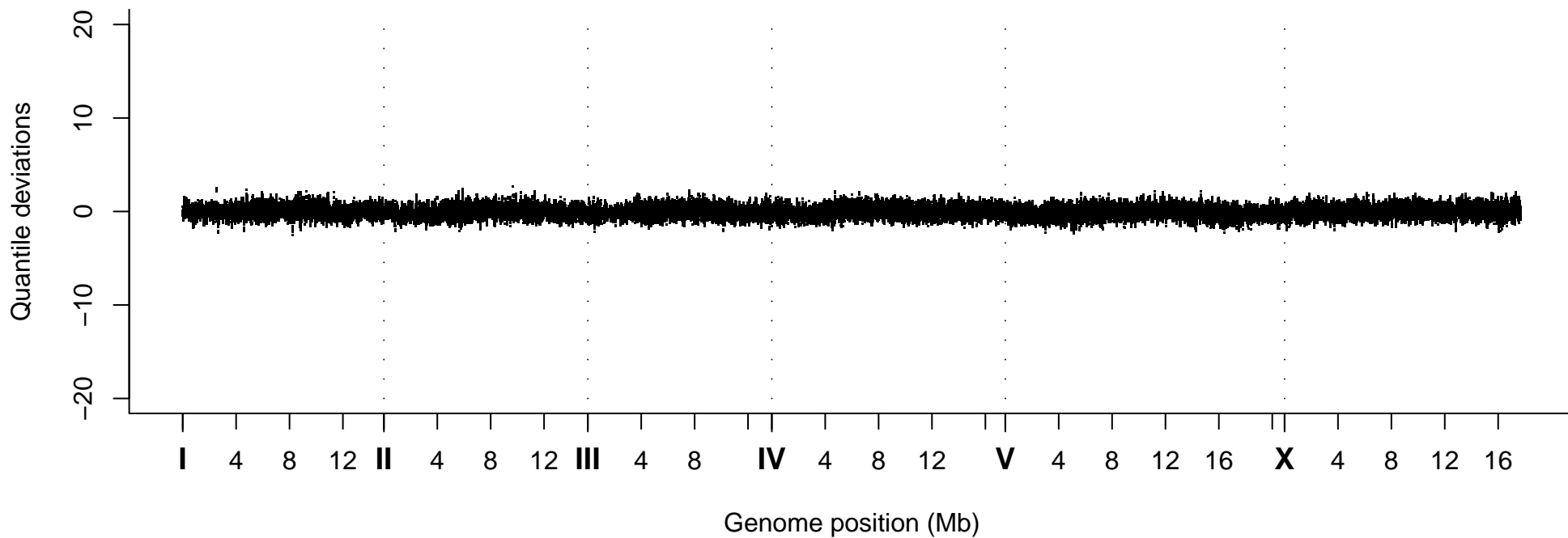
Quantile Deviations, Strain VC40079
