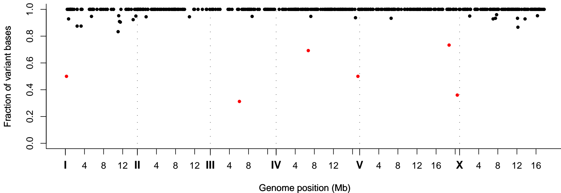
Fraction of Variant Bases at Position, Strain VC40079
