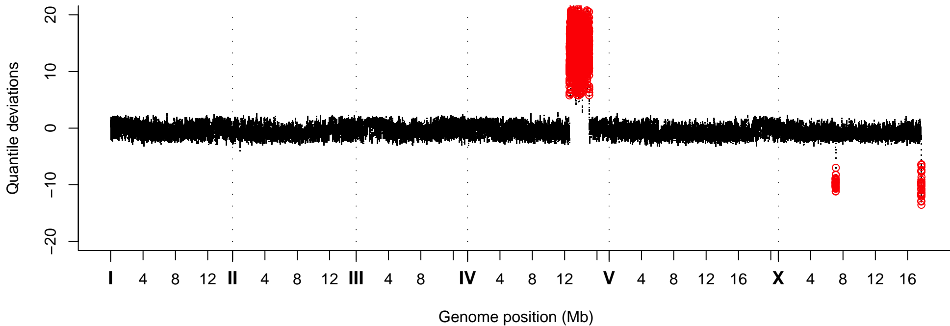
Quantile Deviations, Strain VC40082
