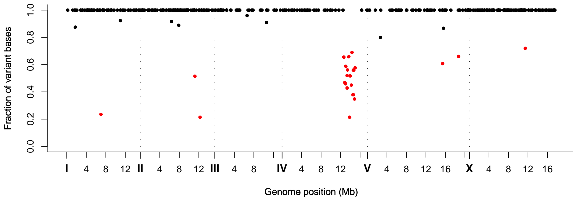
Fraction of Variant Bases at Position, Strain VC40082
