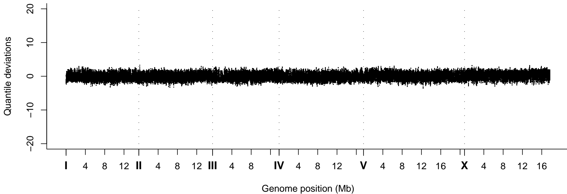
Quantile Deviations, Strain VC40083
