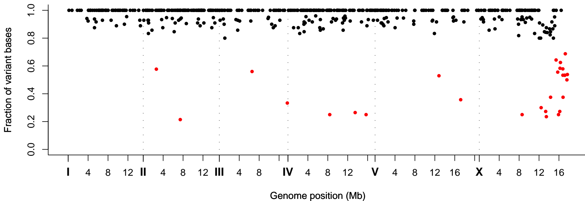
Fraction of Variant Bases at Position, Strain VC40083
