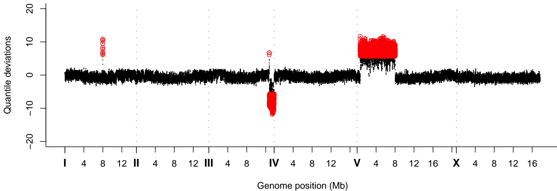
Quantile Deviations, Strain VC40084
