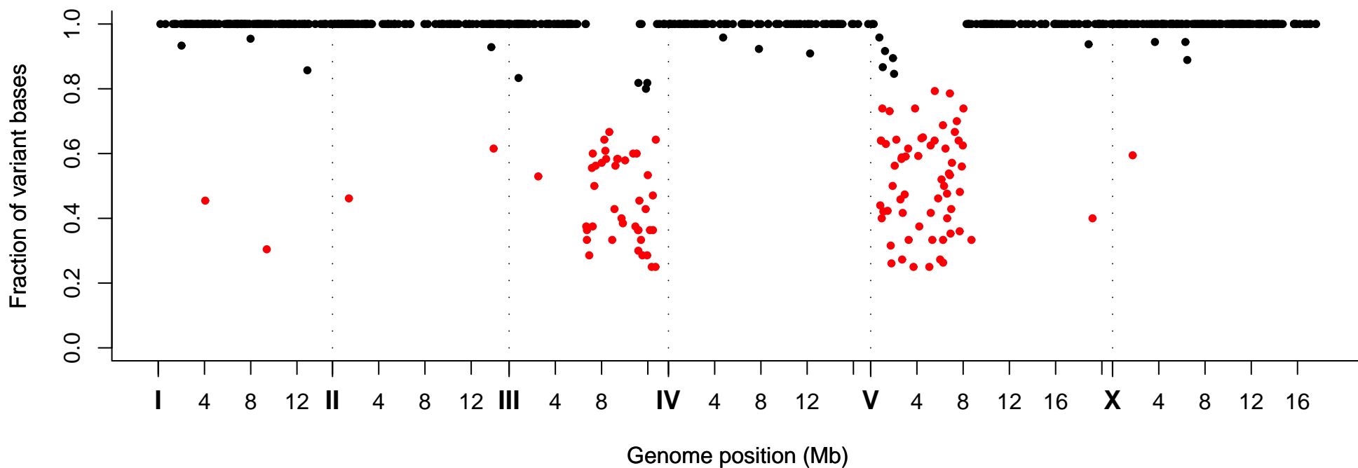
Fraction of Variant Bases at Position, Strain VC40084
