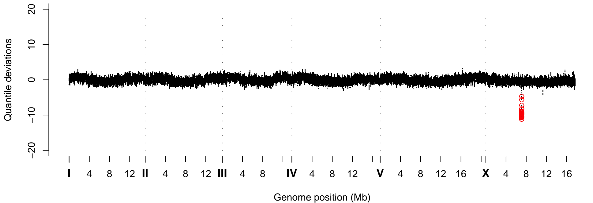
Quantile Deviations, Strain VC40088
