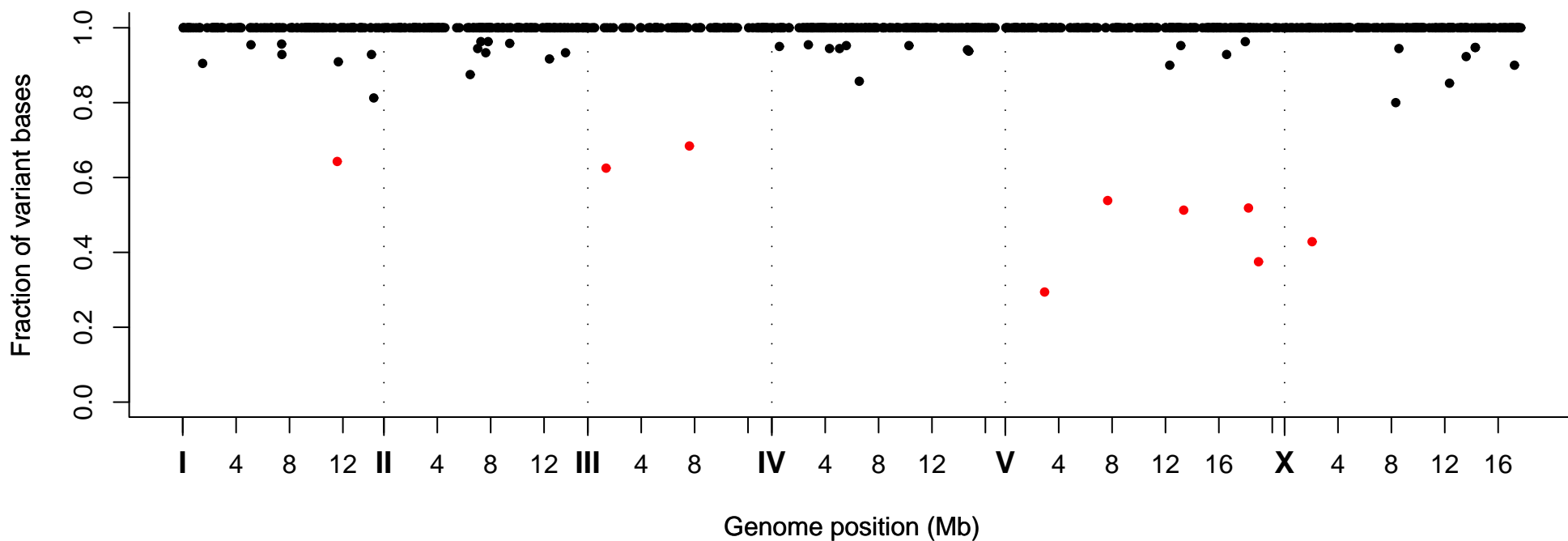
Fraction of Variant Bases at Position, Strain VC40088
