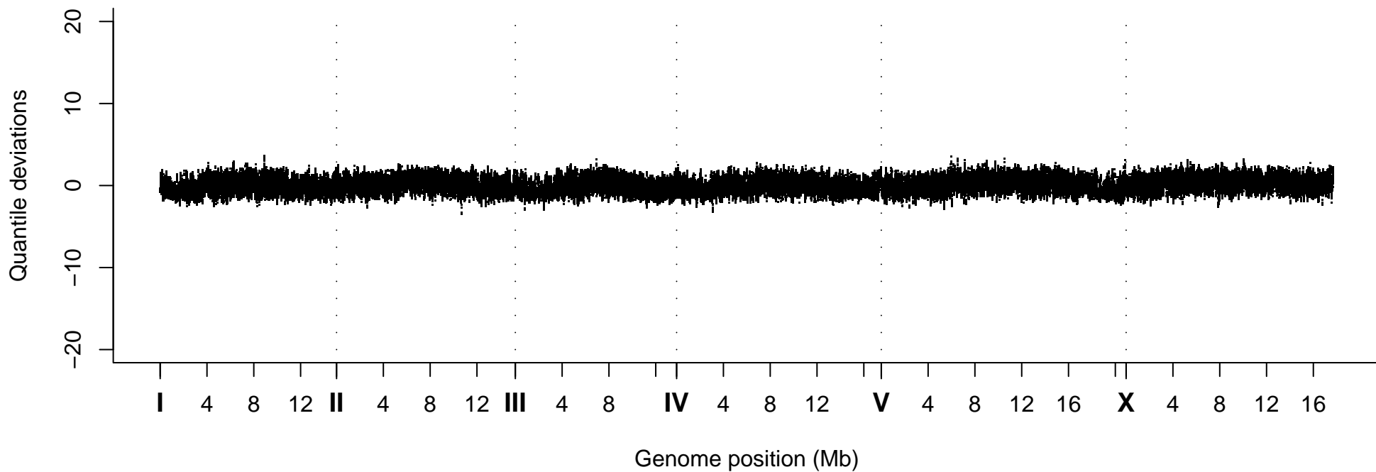
Quantile Deviations, Strain VC40091
