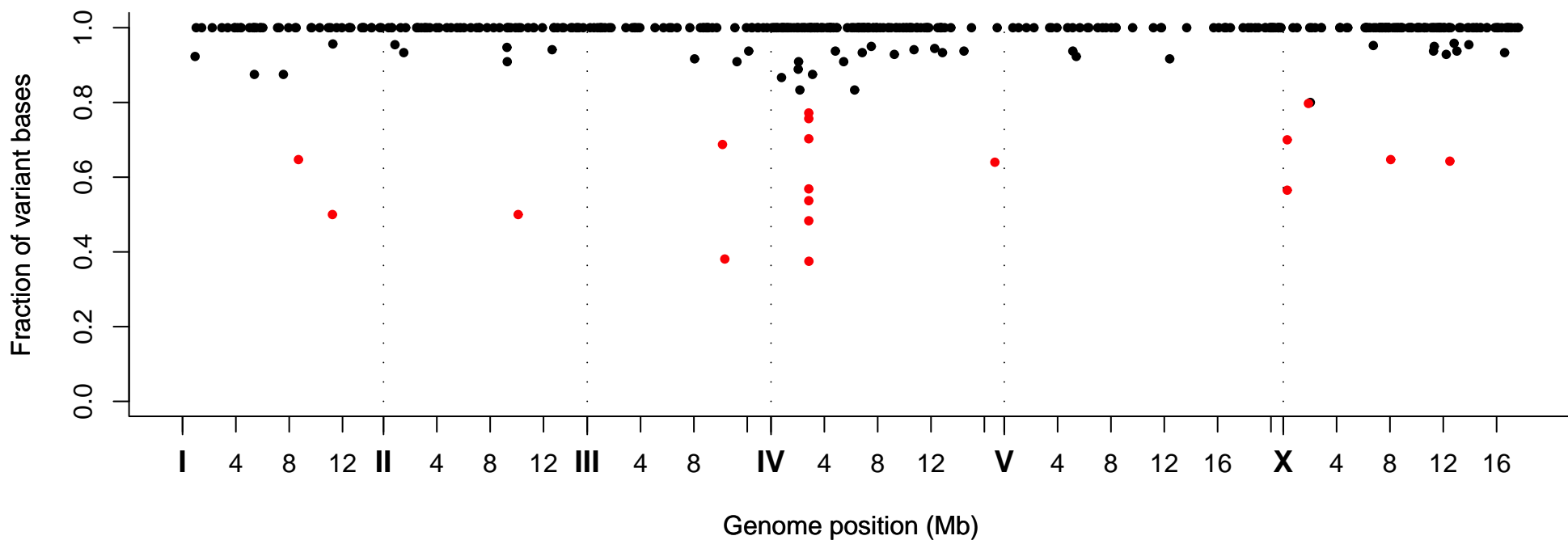
Fraction of Variant Bases at Position, Strain VC40091
