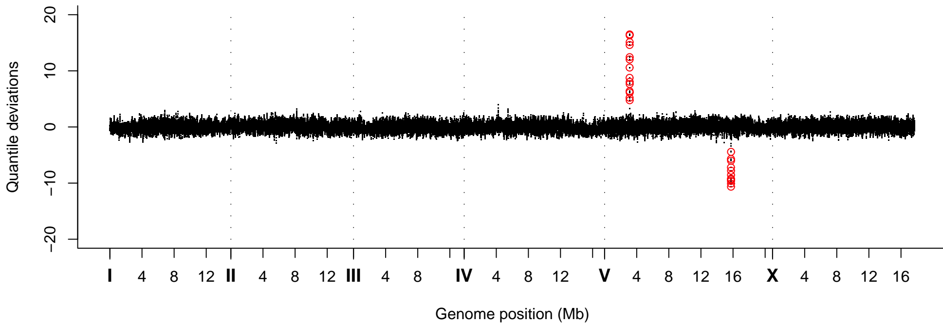
Quantile Deviations, Strain VC40092
