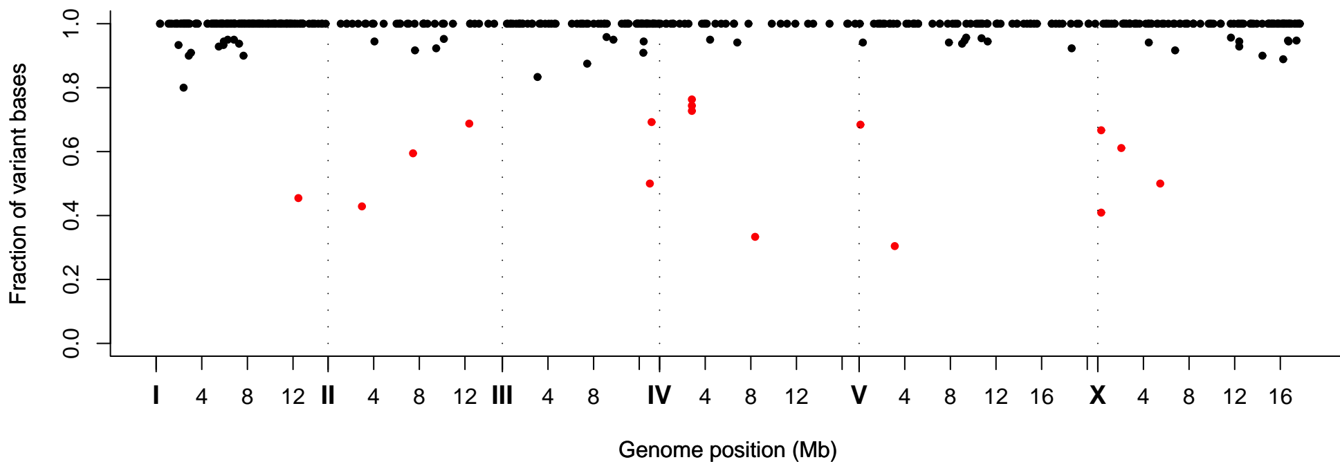
Fraction of Variant Bases at Position, Strain VC40092
