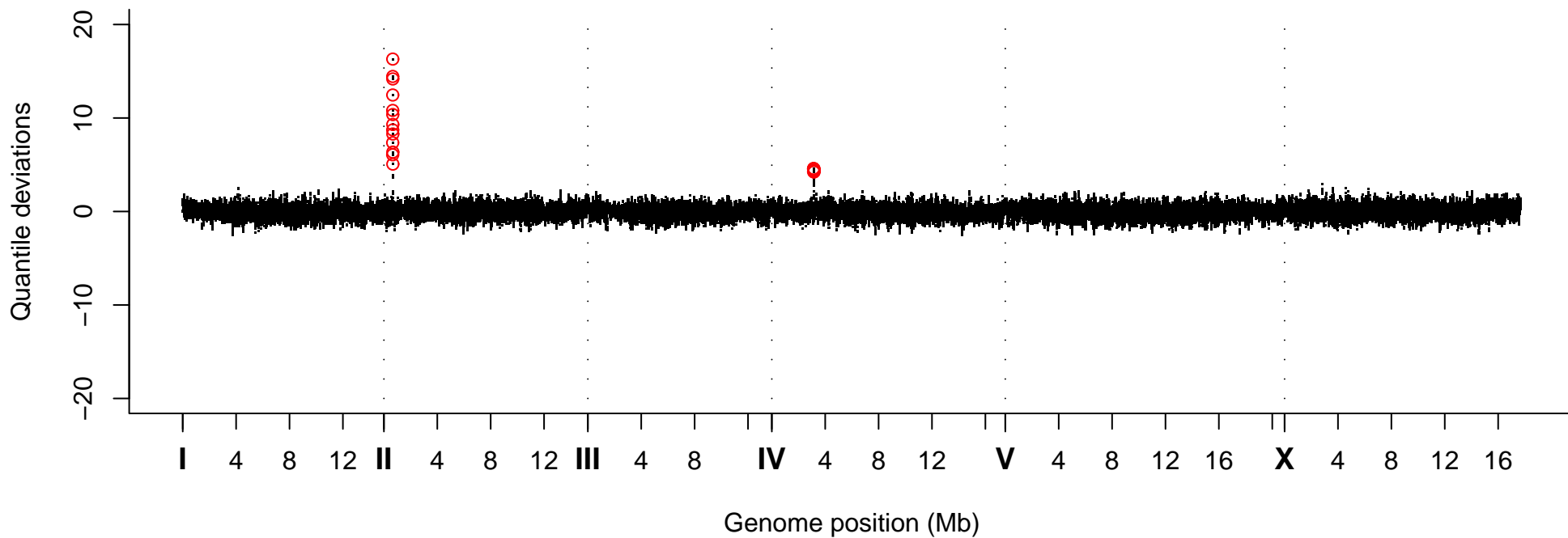
Quantile Deviations, Strain VC40094
