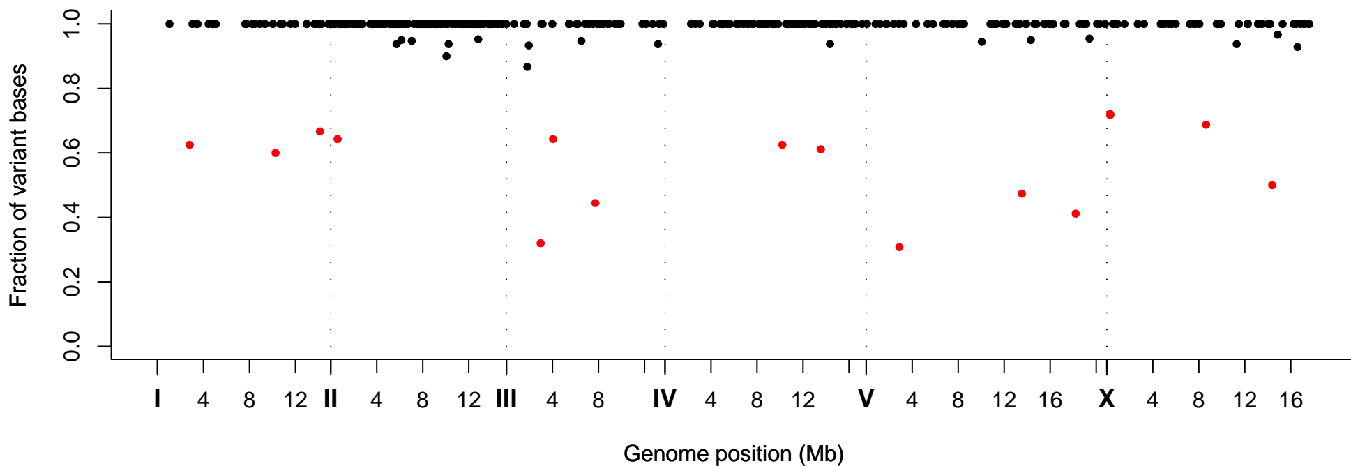
Fraction of Variant Bases at Position, Strain VC40094
