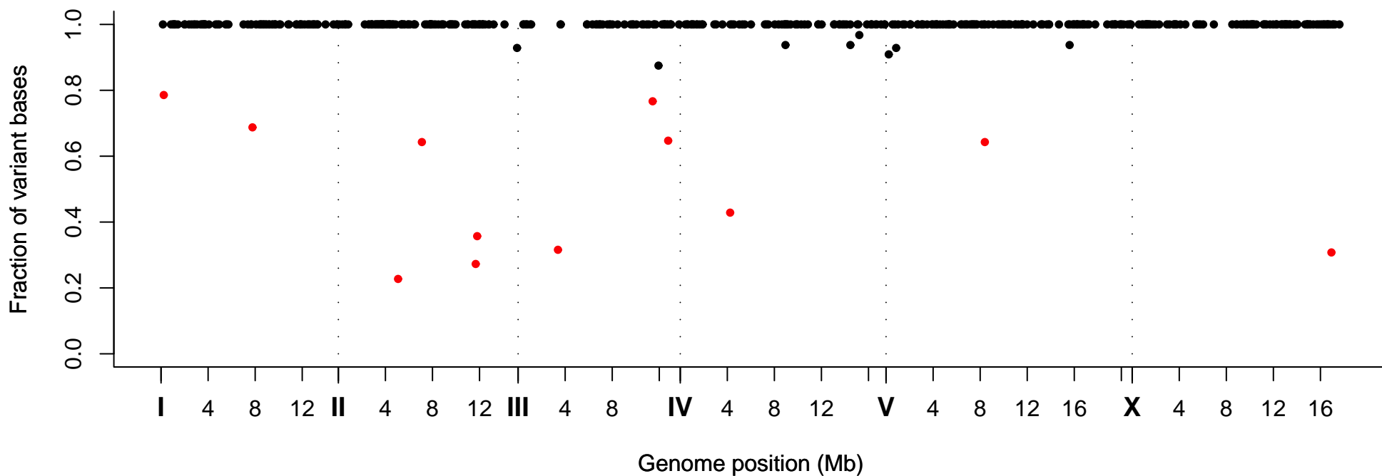
Fraction of Variant Bases at Position, Strain VC40095
