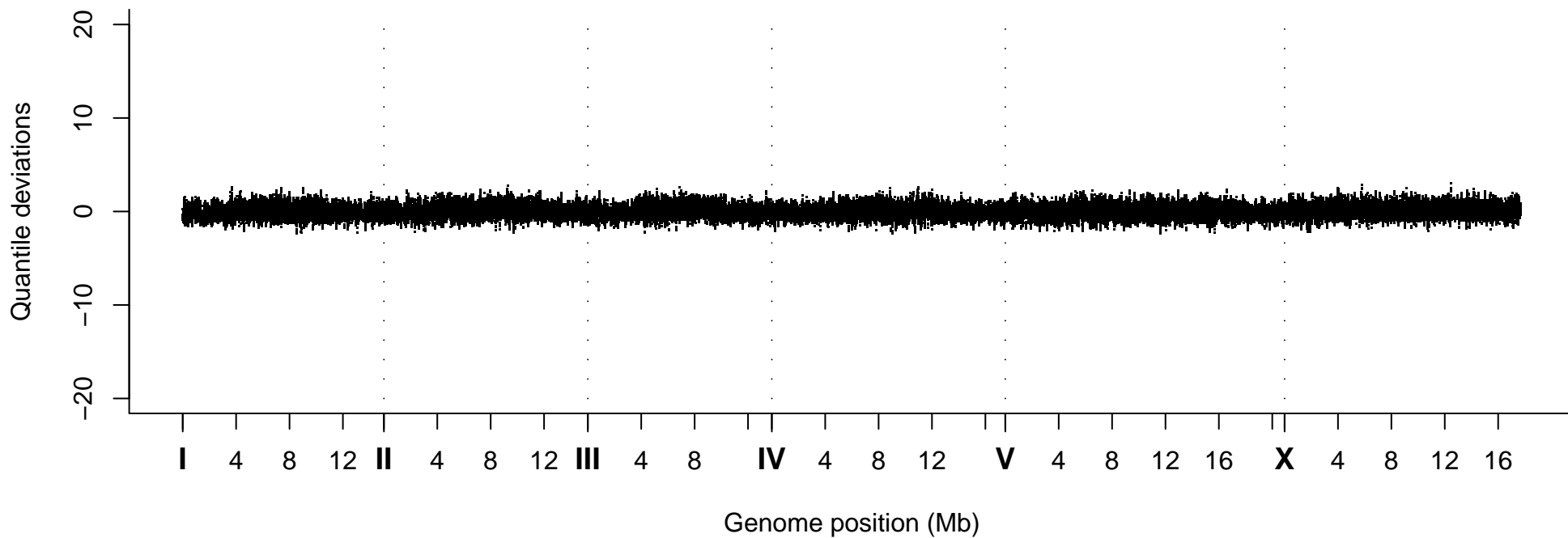
Quantile Deviations, Strain VC40095
