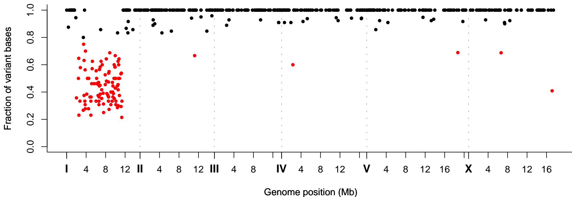
Fraction of Variant Bases at Position, Strain VC40098
