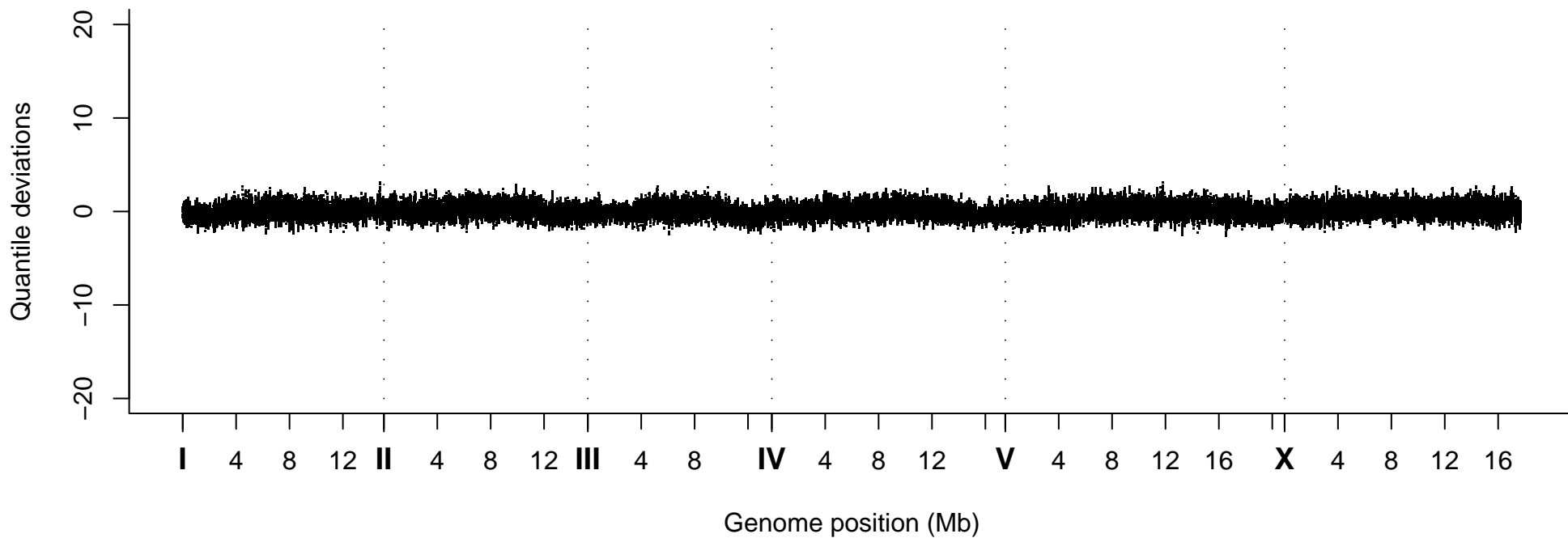
Quantile Deviations, Strain VC40098
