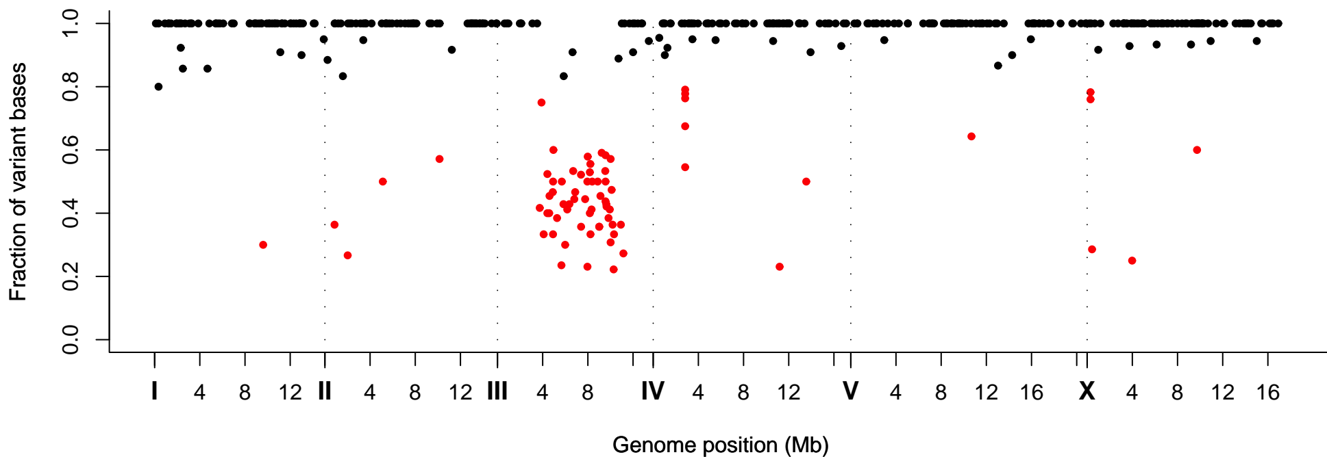
Fraction of Variant Bases at Position, Strain VC40101
