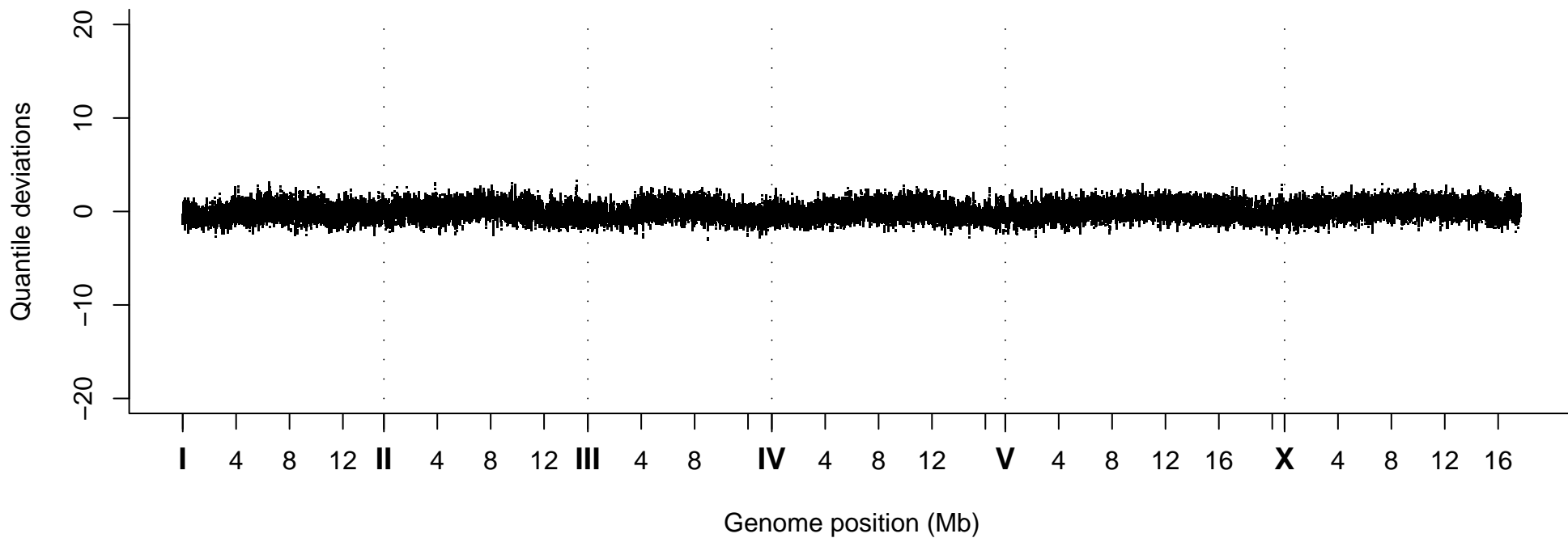
Quantile Deviations, Strain VC40101
