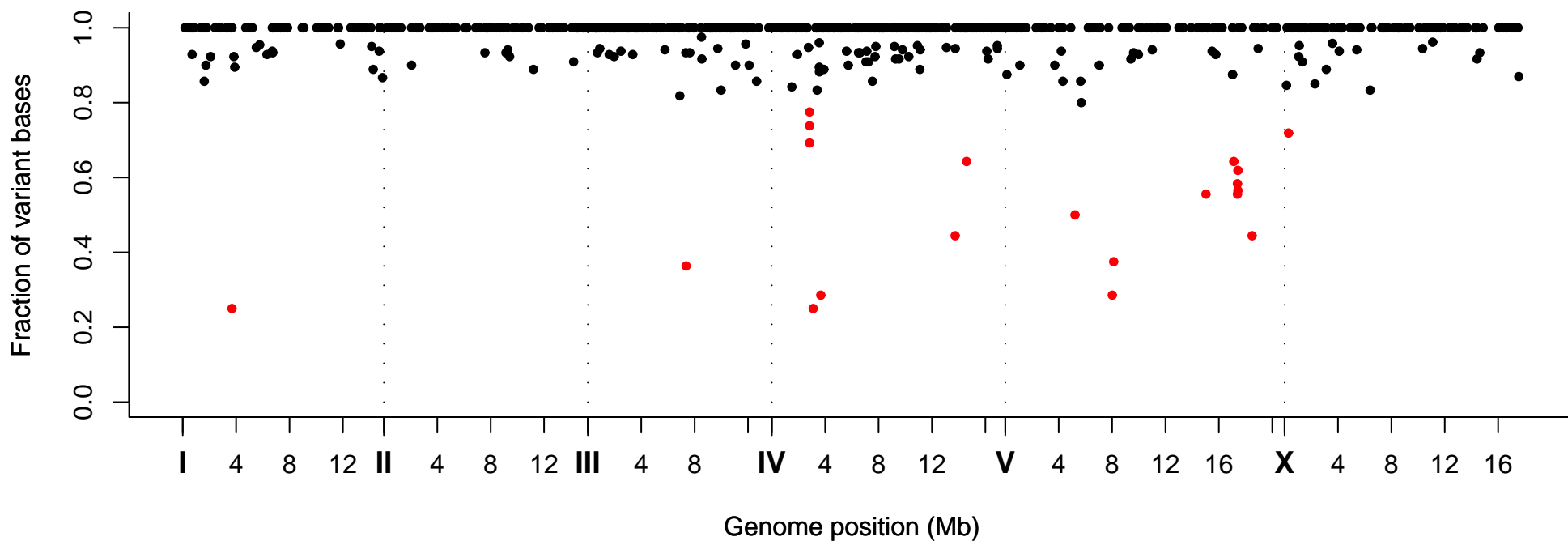
Fraction of Variant Bases at Position, Strain VC40102
