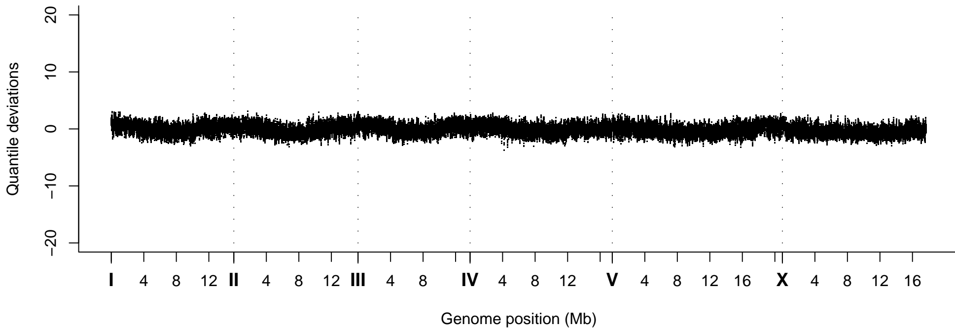
Quantile Deviations, Strain VC40102
