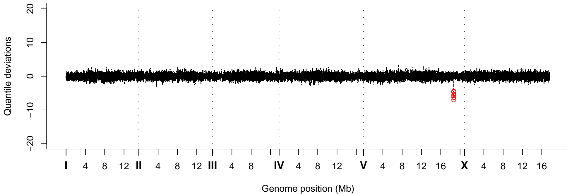
Quantile Deviations, Strain VC40113
