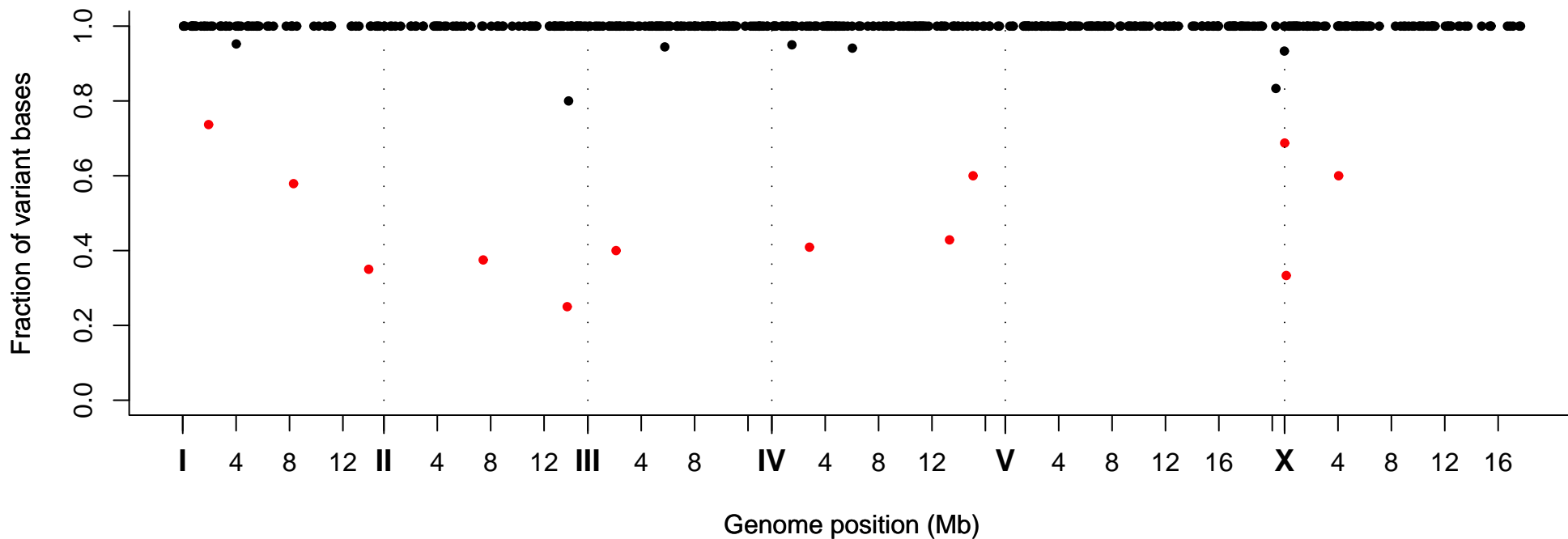
Fraction of Variant Bases at Position, Strain VC40113
