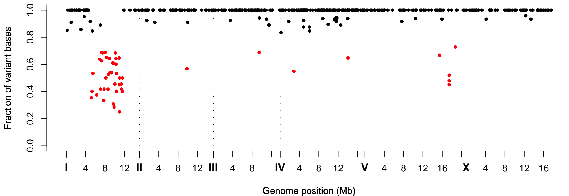
Fraction of Variant Bases at Position, Strain VC40114
