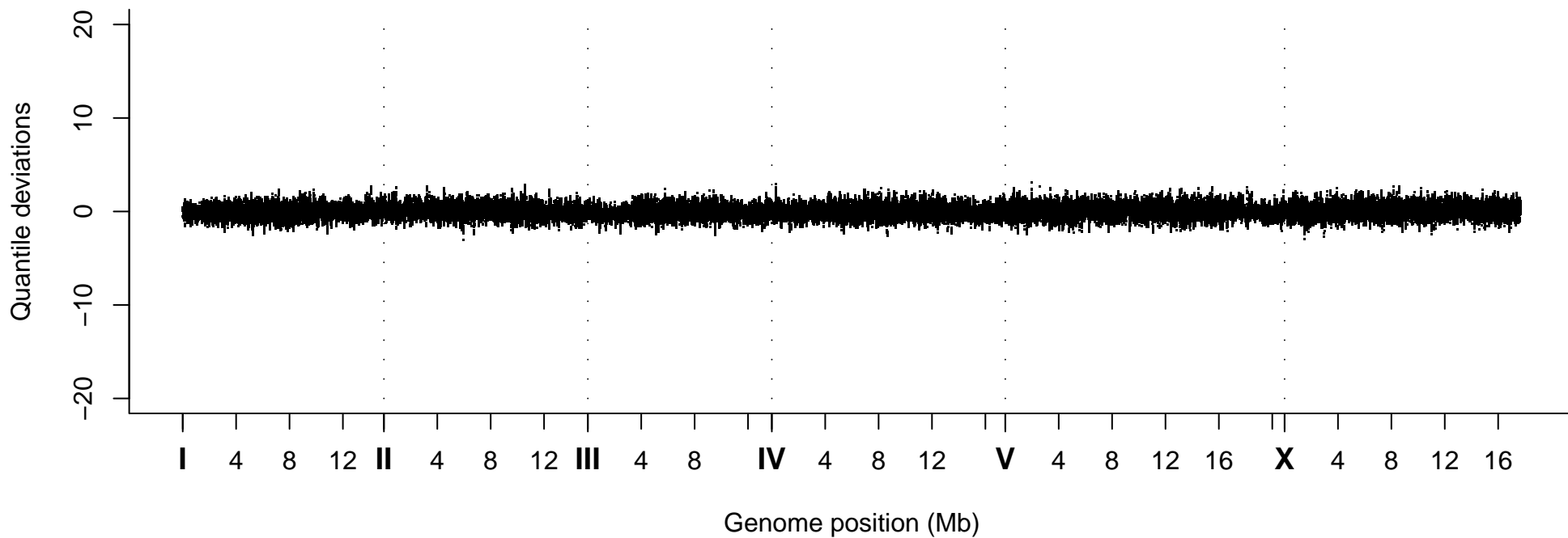
Quantile Deviations, Strain VC40114
