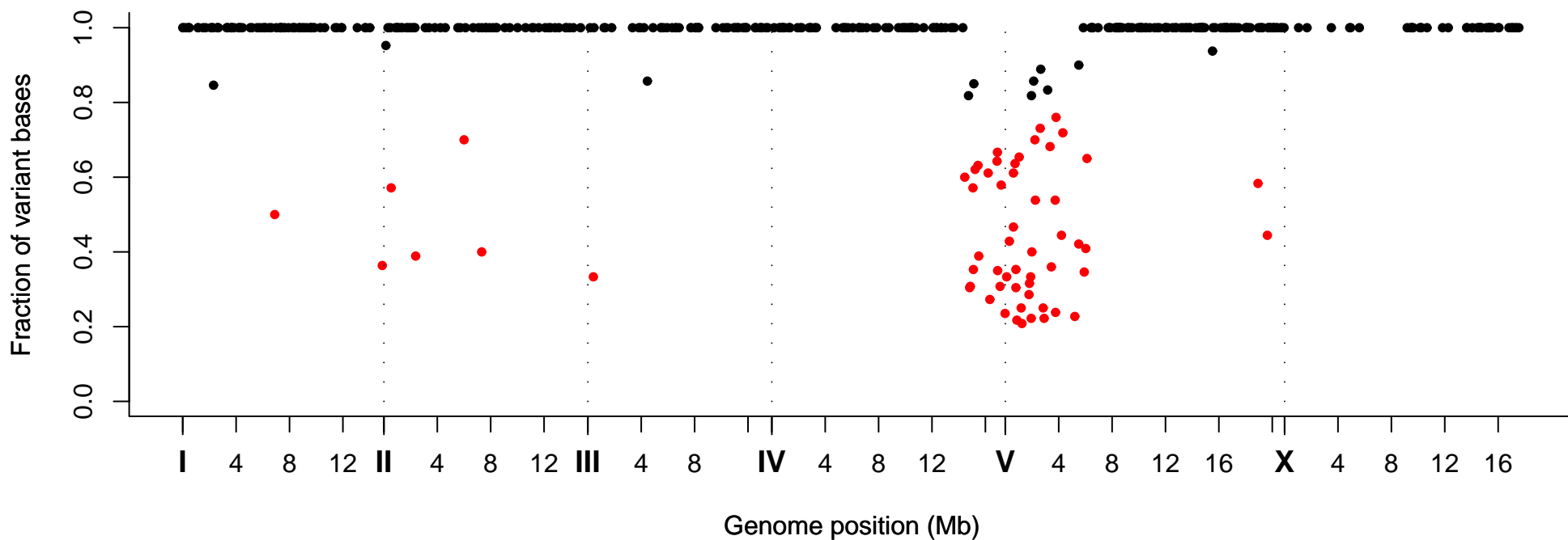
Fraction of Variant Bases at Position, Strain VC40117
