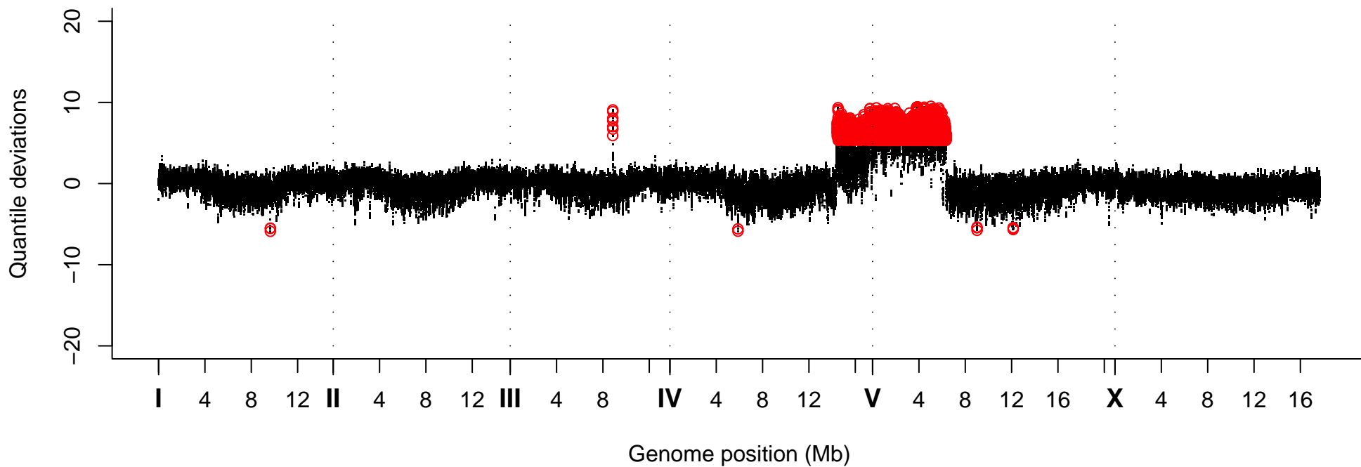
Quantile Deviations, Strain VC40117
