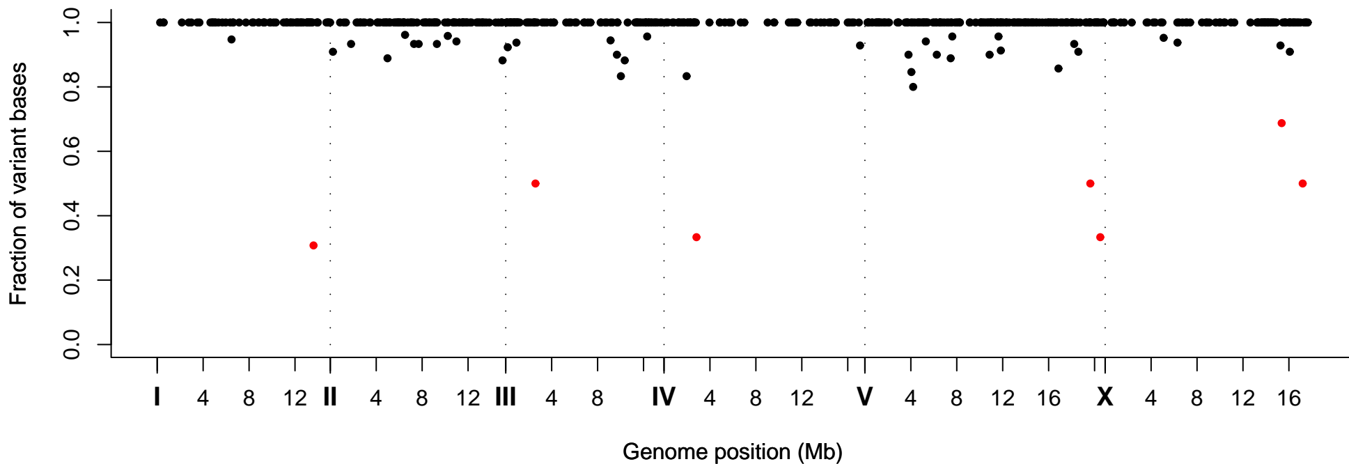
Fraction of Variant Bases at Position, Strain VC40118
