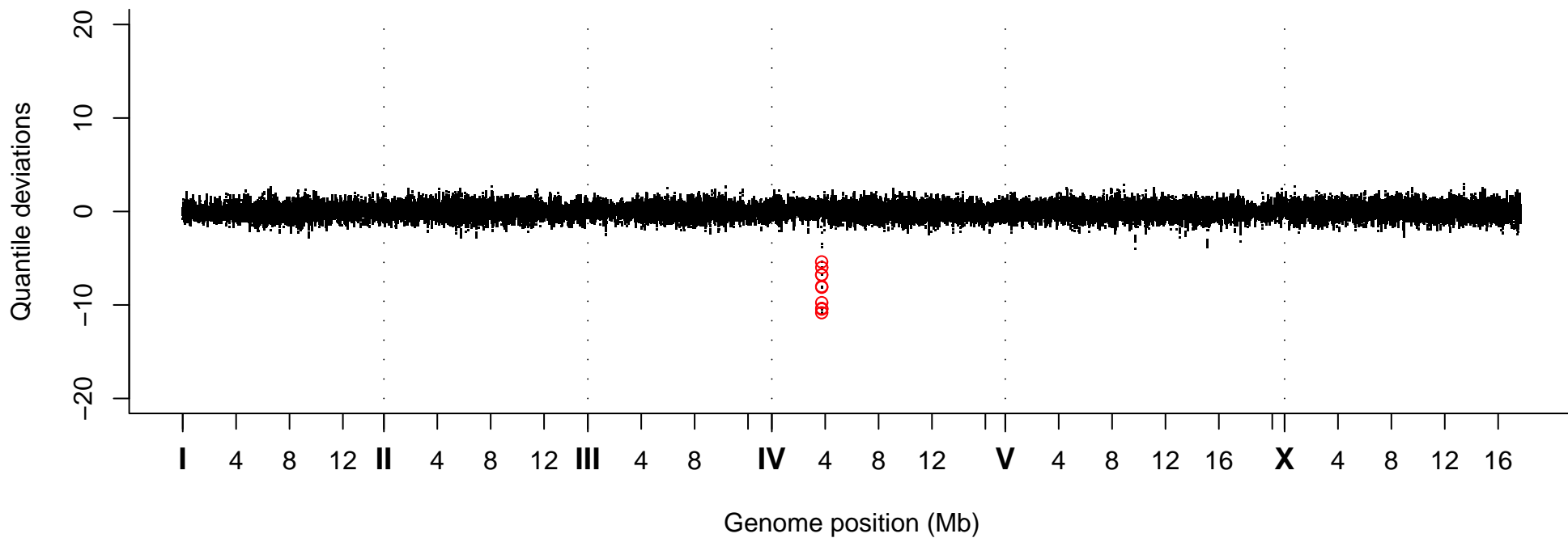
Quantile Deviations, Strain VC40118
