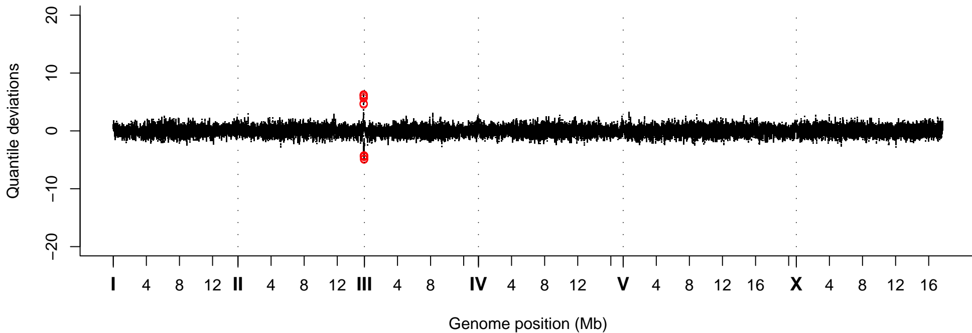
Quantile Deviations, Strain VC40119
