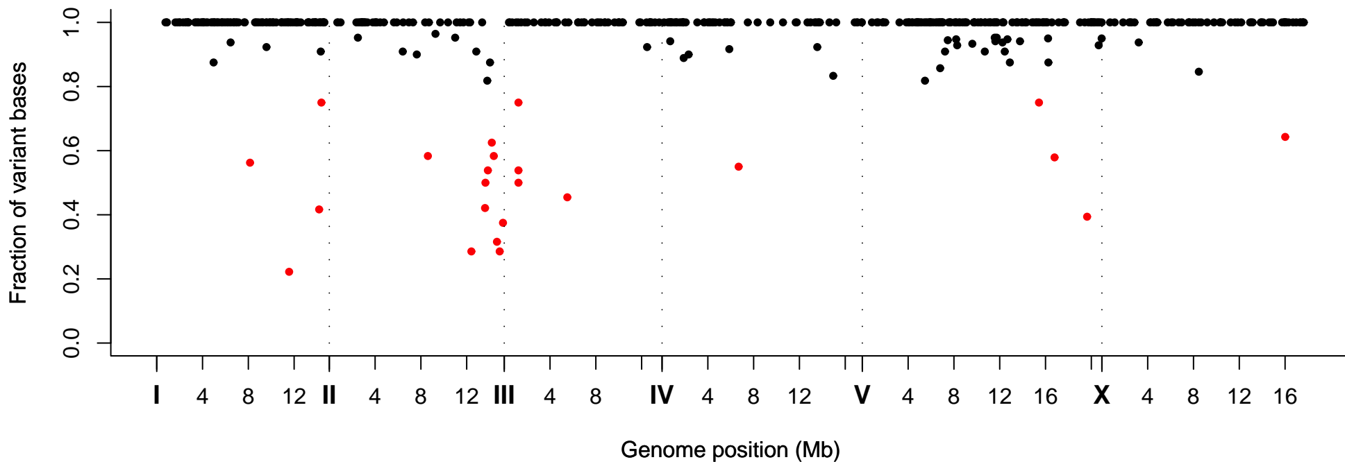
Fraction of Variant Bases at Position, Strain VC40119
