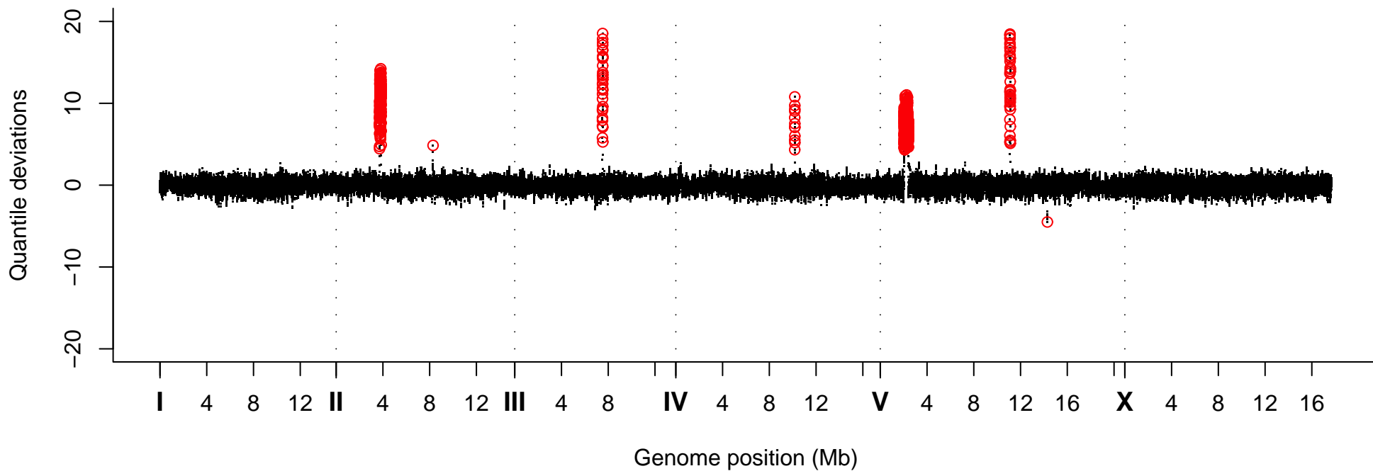
Quantile Deviations, Strain VC40124
