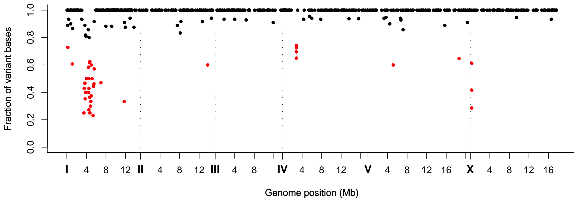
Fraction of Variant Bases at Position, Strain VC40124
