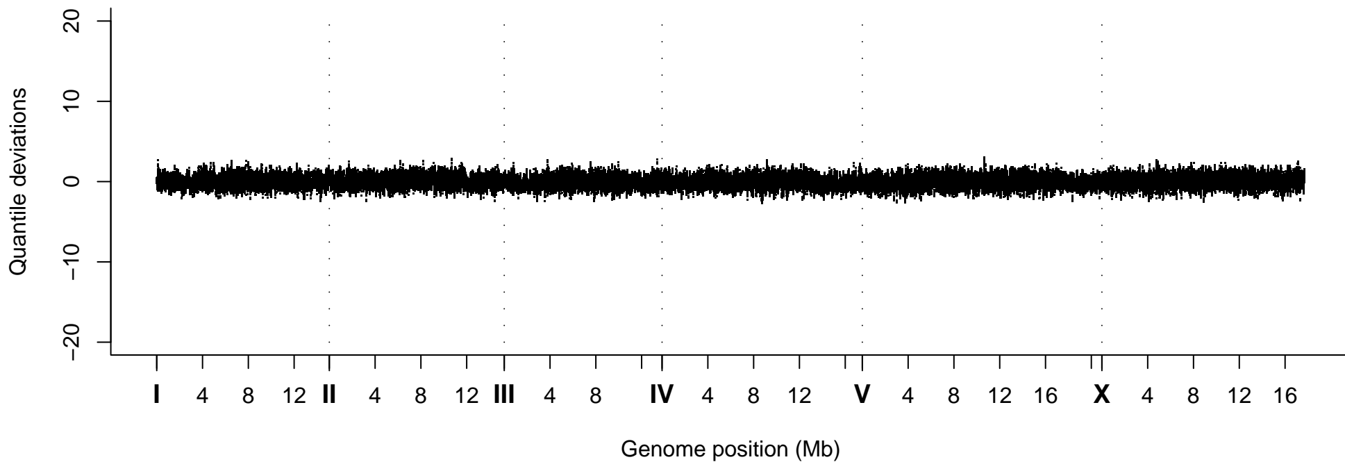
Quantile Deviations, Strain VC40126
