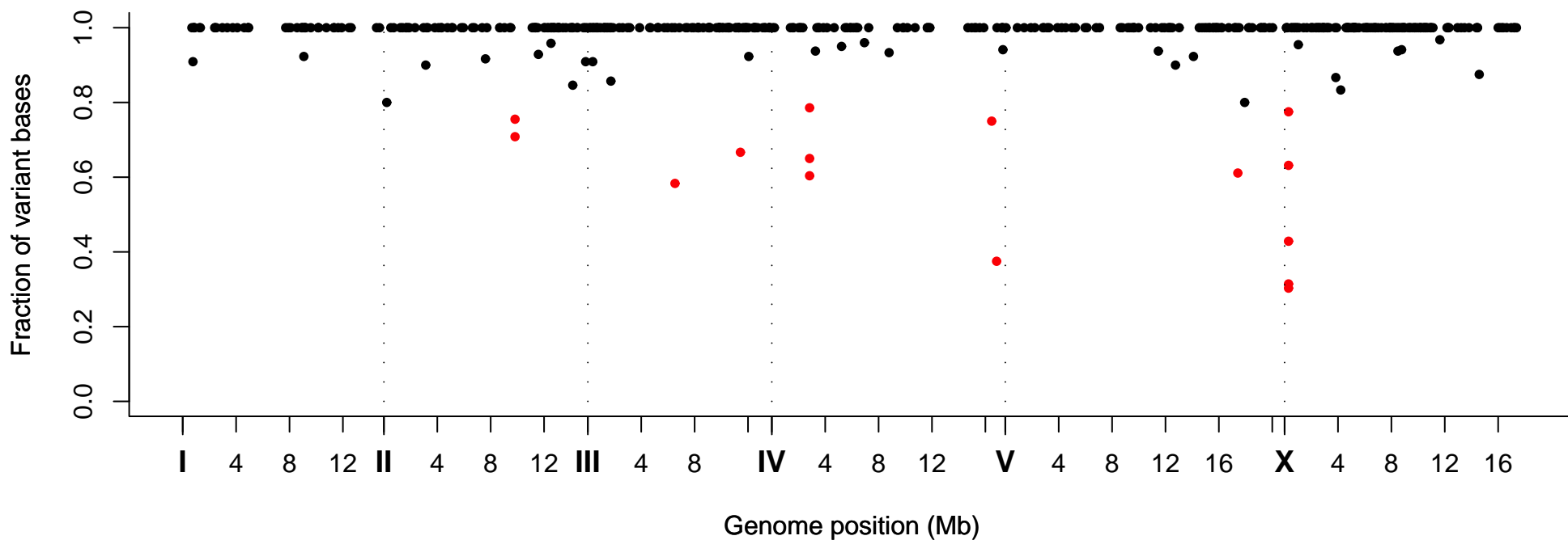
Fraction of Variant Bases at Position, Strain VC40126
