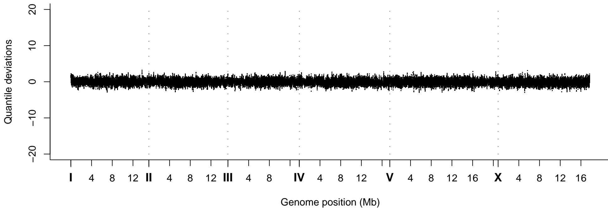
Quantile Deviations, Strain VC40131
