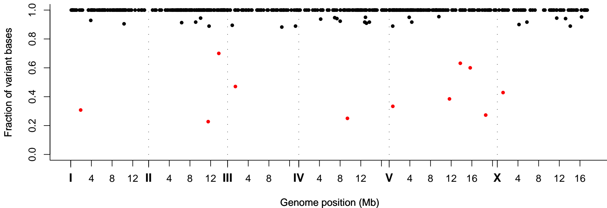
Fraction of Variant Bases at Position, Strain VC40136
