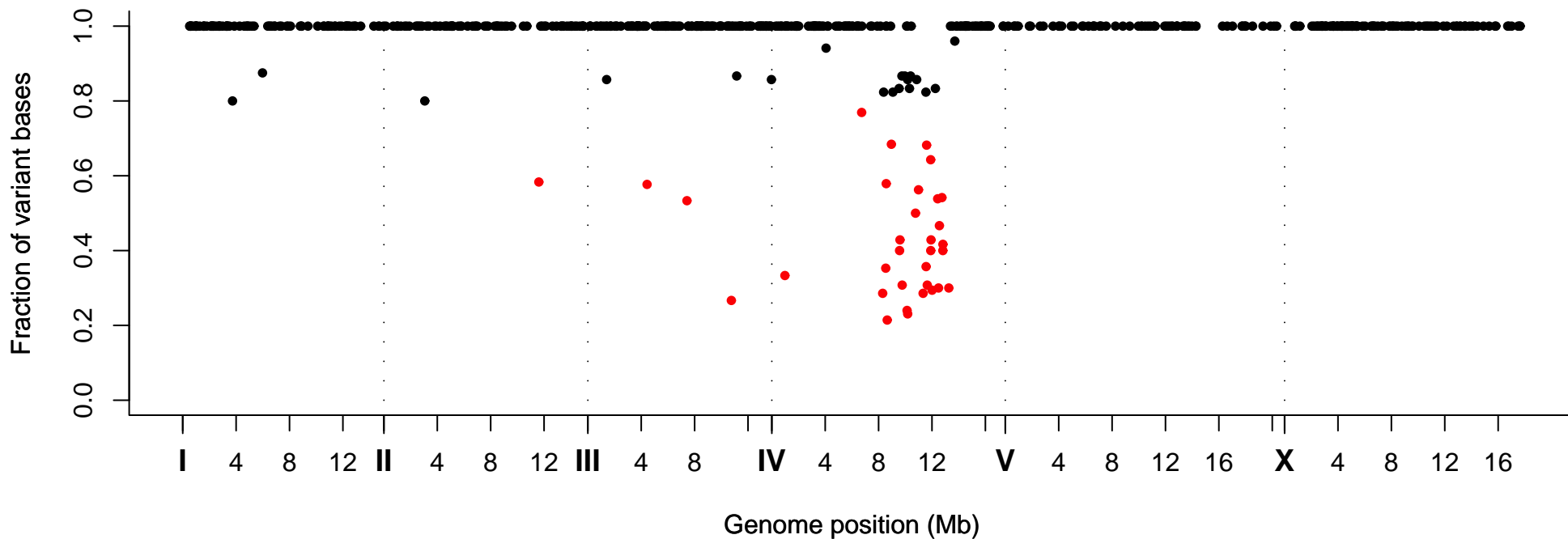
Fraction of Variant Bases at Position, Strain VC40137
