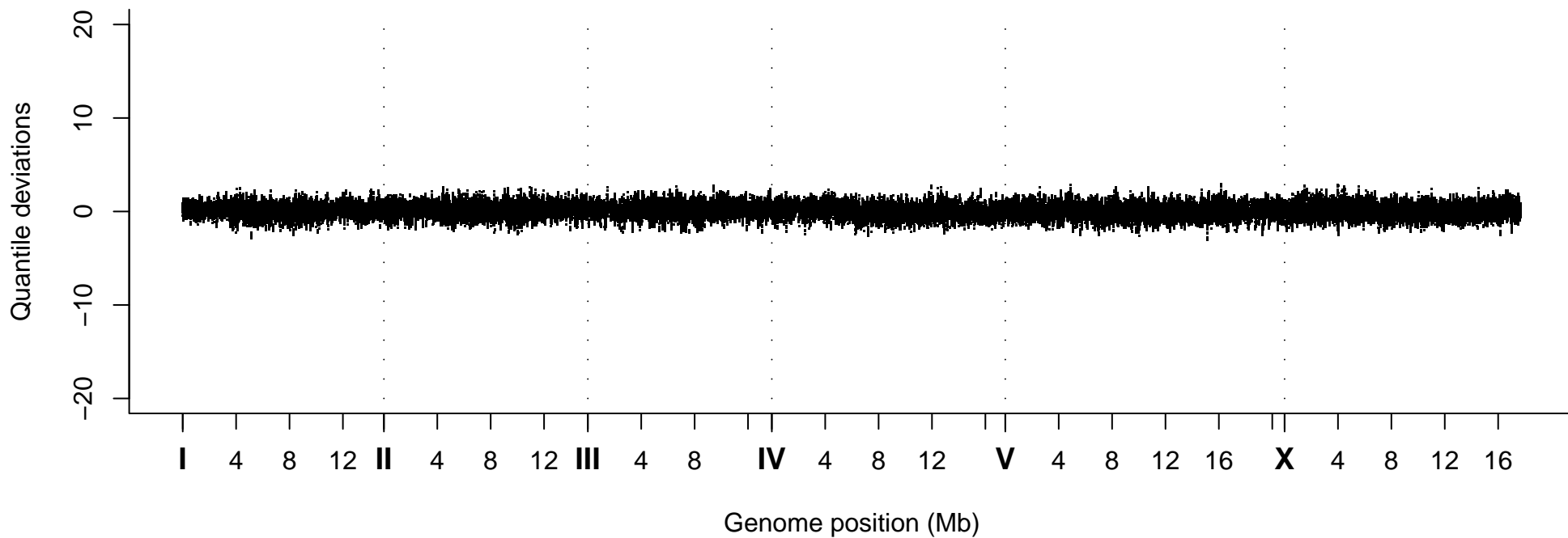
Quantile Deviations, Strain VC40137
