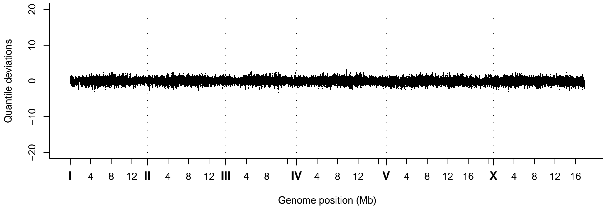
Quantile Deviations, Strain VC40141
