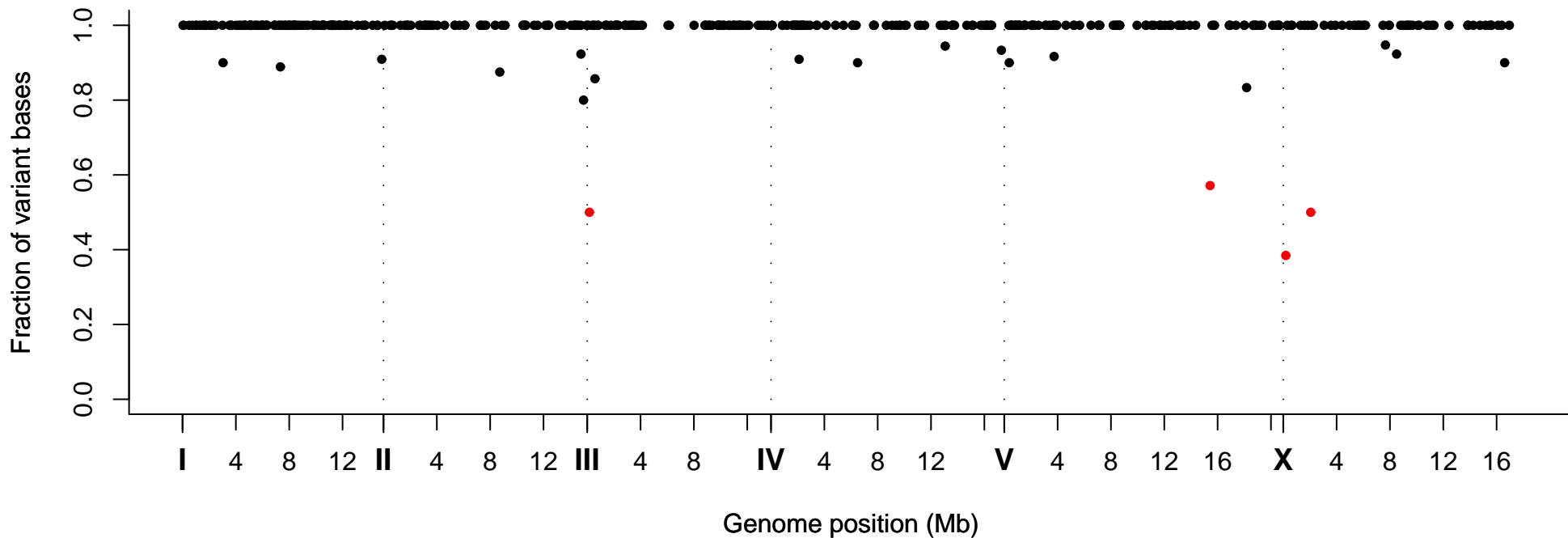
Fraction of Variant Bases at Position, Strain VC40141
