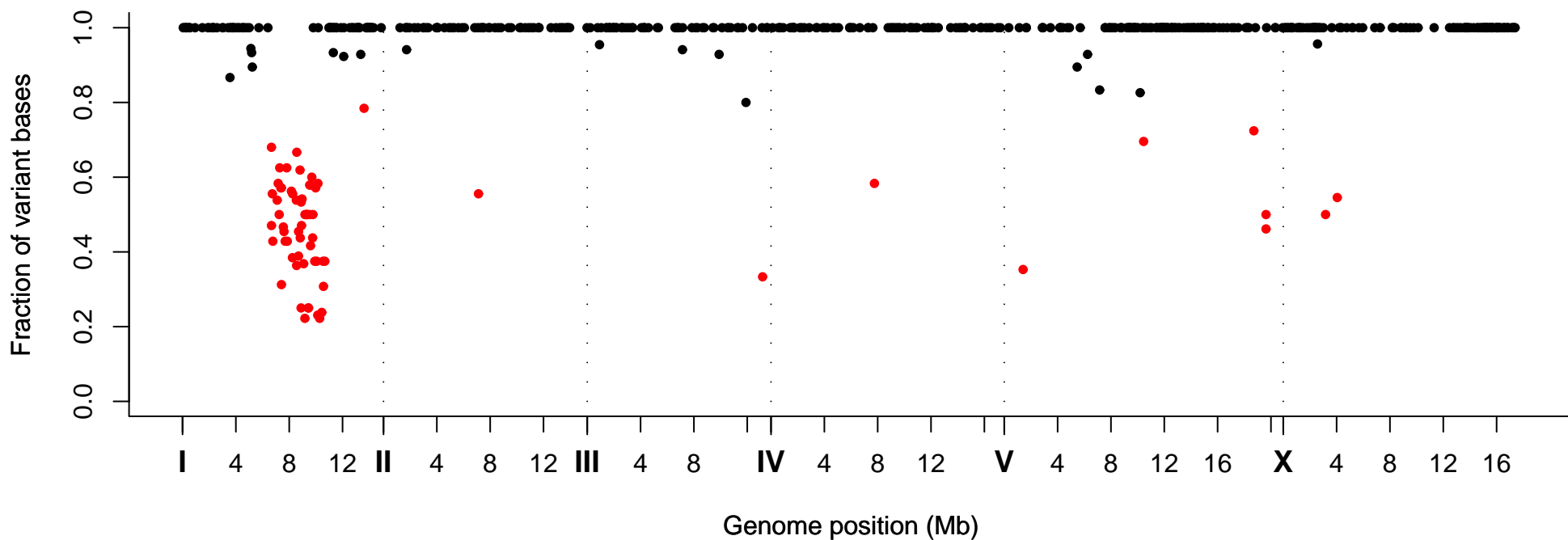
Fraction of Variant Bases at Position, Strain VC40148
