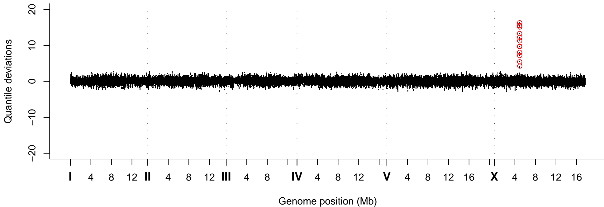
Quantile Deviations, Strain VC40148
