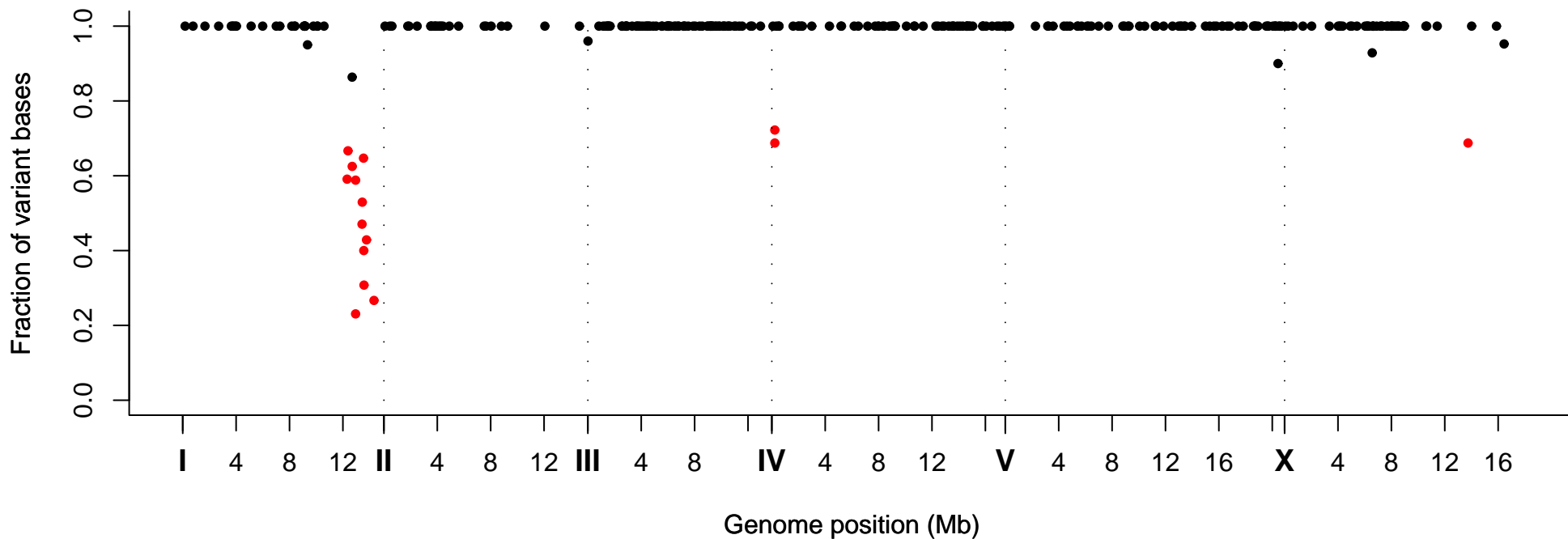
Fraction of Variant Bases at Position, Strain VC40152
