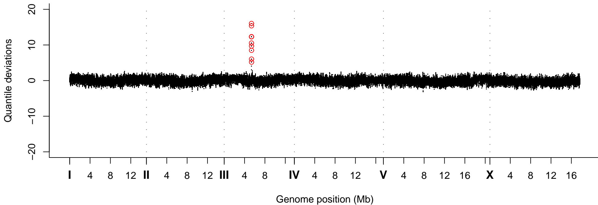
Quantile Deviations, Strain VC40152
