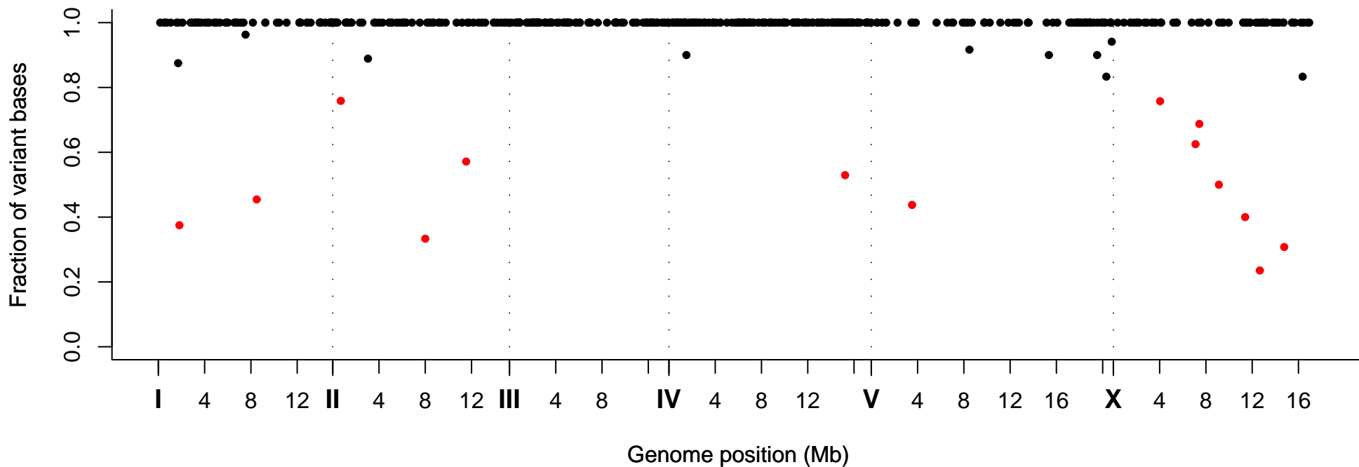
Fraction of Variant Bases at Position, Strain VC40157
