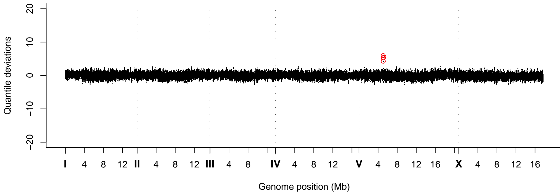
Quantile Deviations, Strain VC40157
