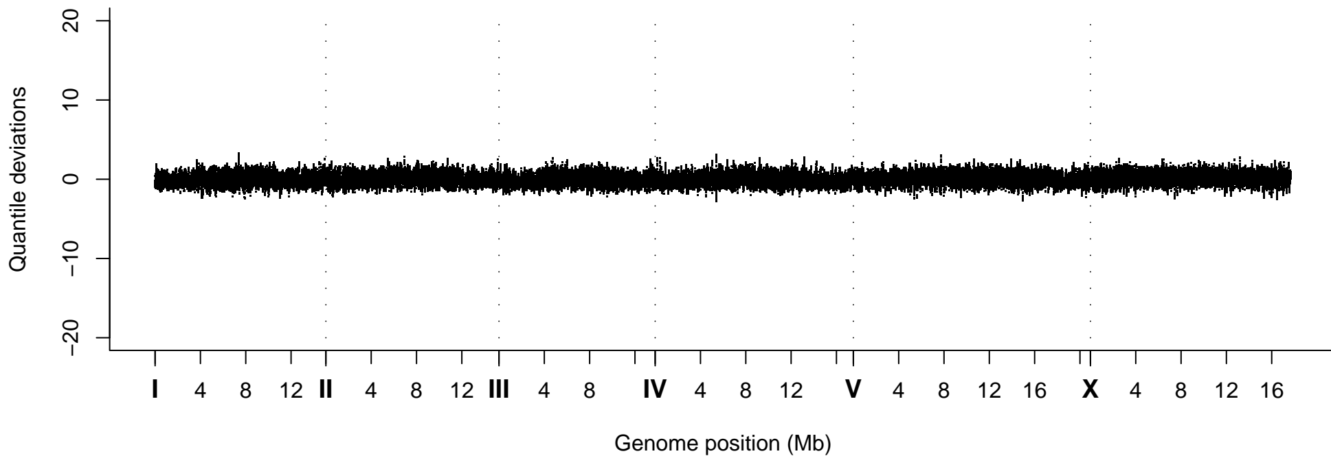
Quantile Deviations, Strain VC40164
