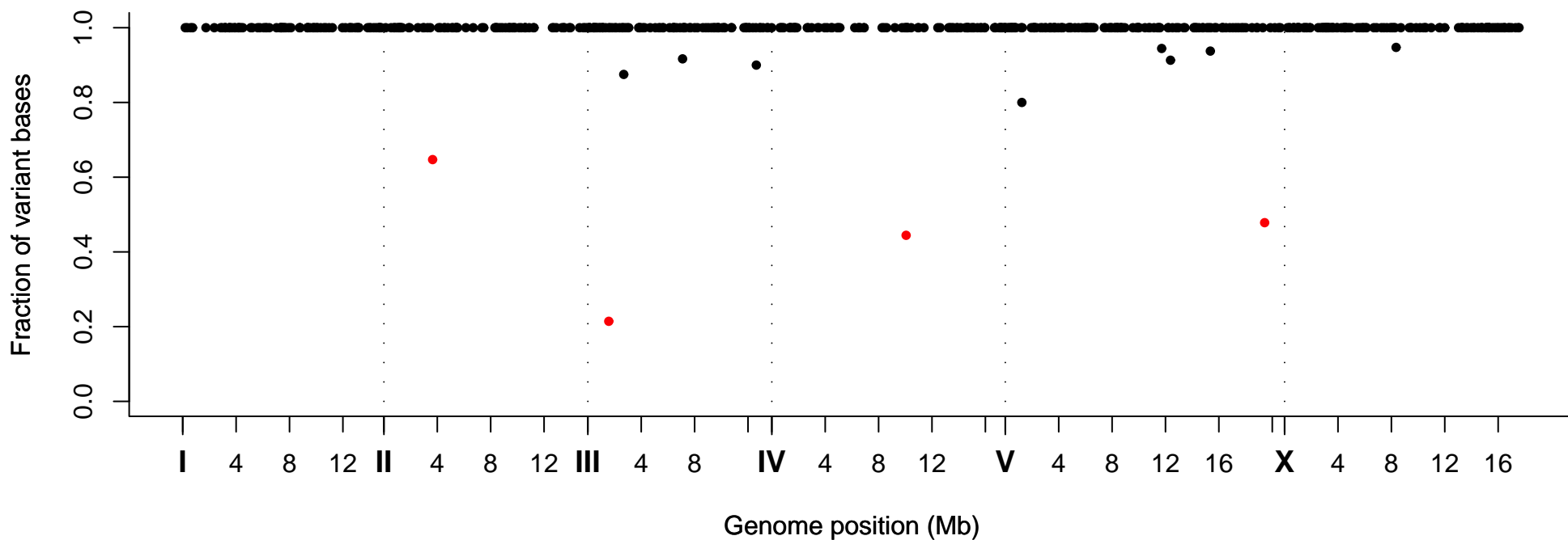
Fraction of Variant Bases at Position, Strain VC40164
