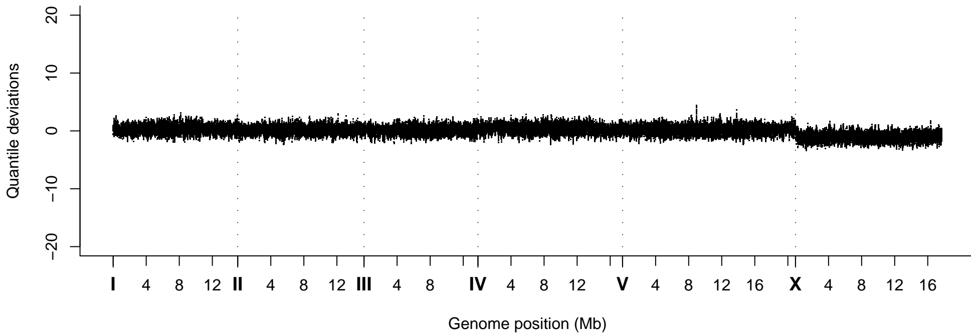
Quantile Deviations, Strain VC40166
