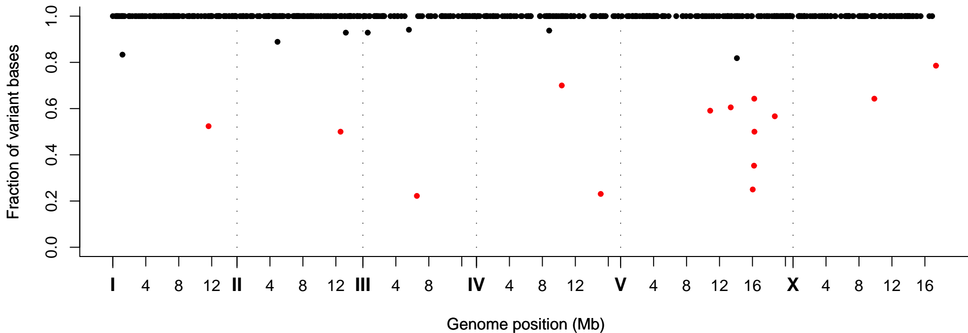
Fraction of Variant Bases at Position, Strain VC40166
