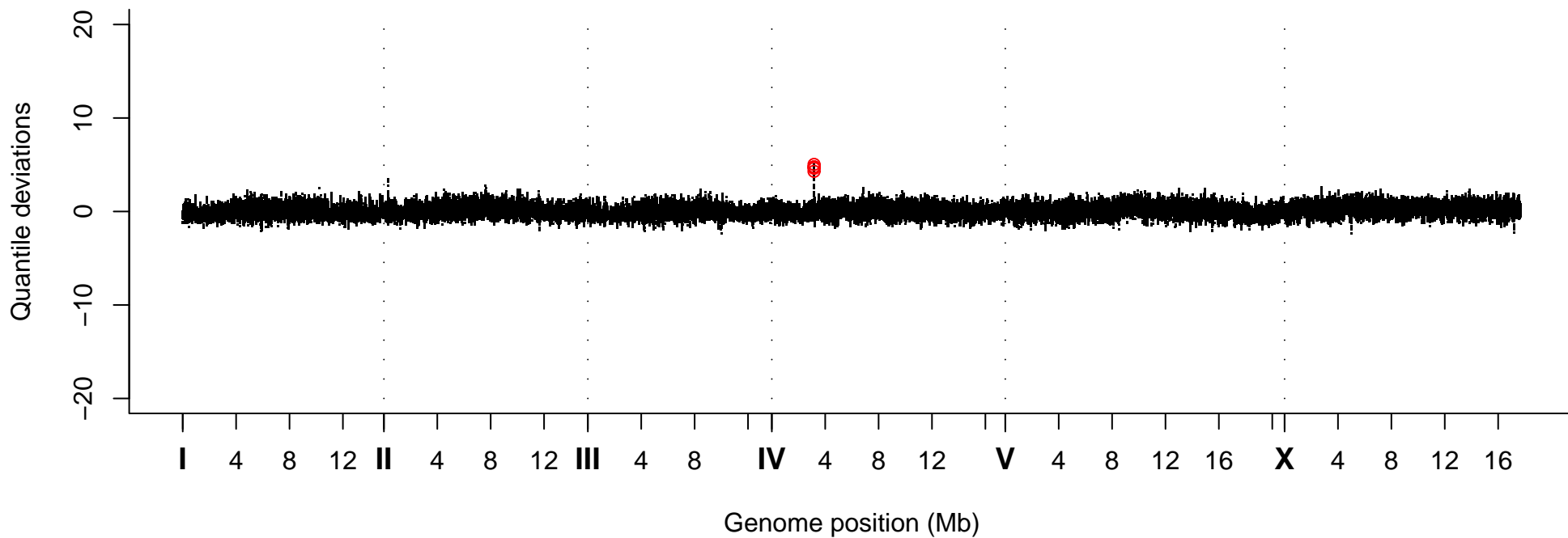
Quantile Deviations, Strain VC40168
