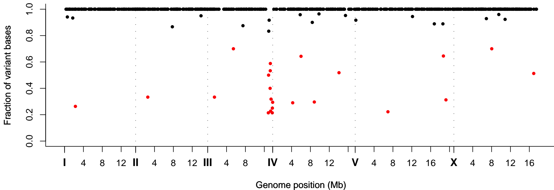
Fraction of Variant Bases at Position, Strain VC40168
