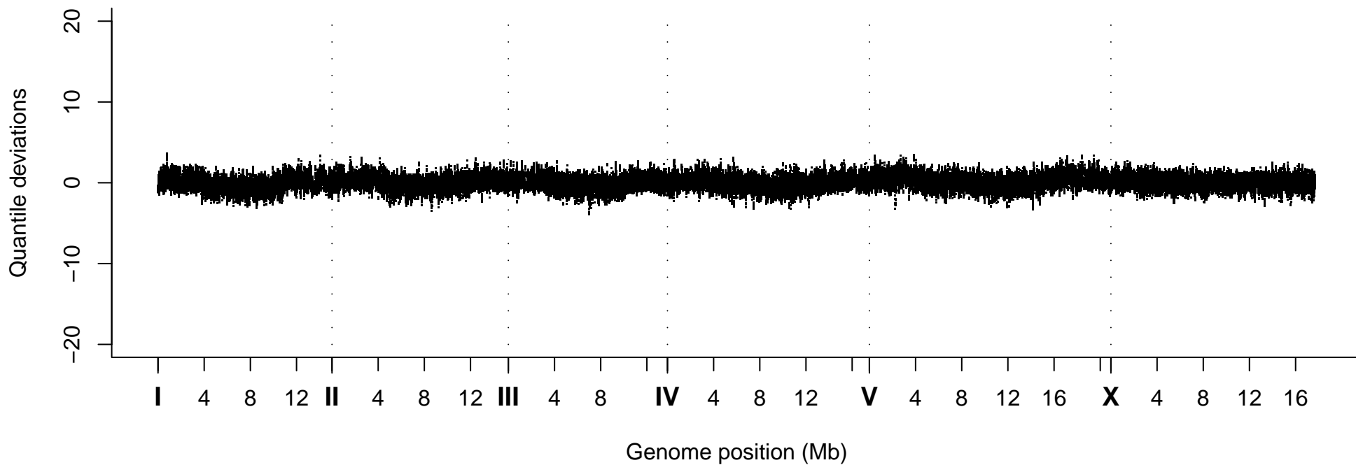
Quantile Deviations, Strain VC40172
