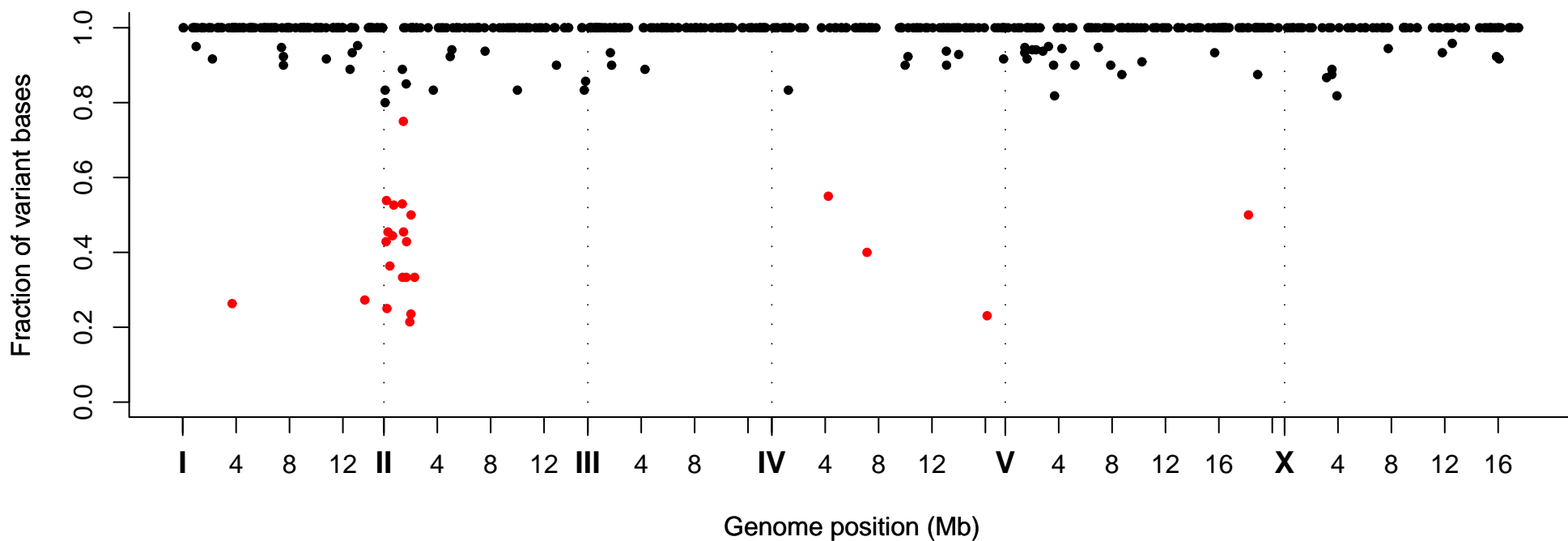
Fraction of Variant Bases at Position, Strain VC40172
