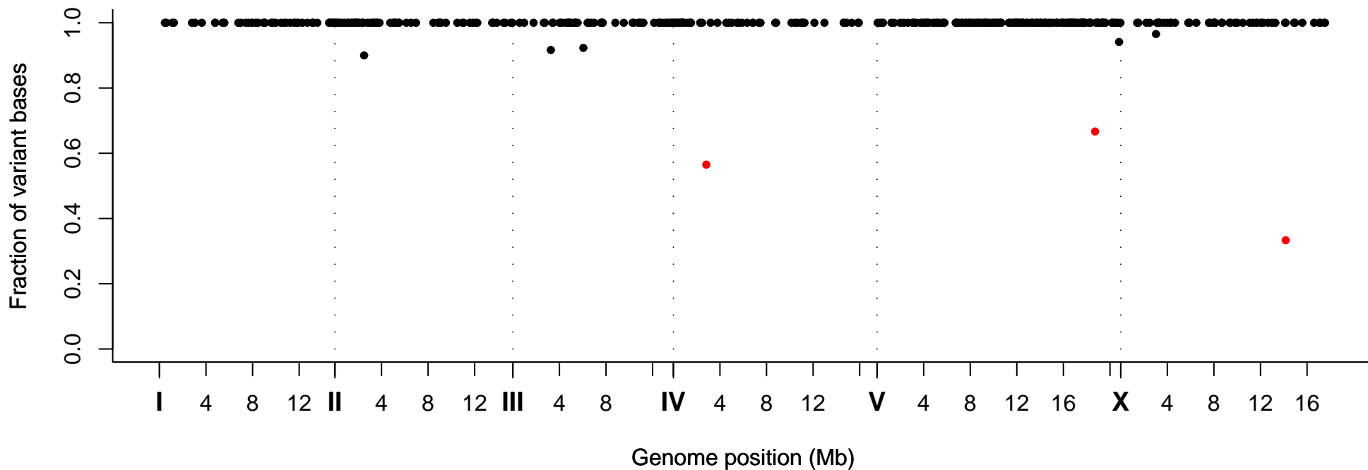
Fraction of Variant Bases at Position, Strain VC40175
