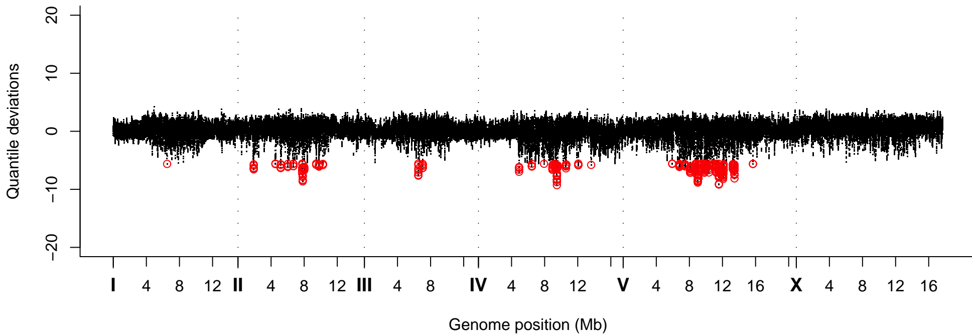
Quantile Deviations, Strain VC40175
