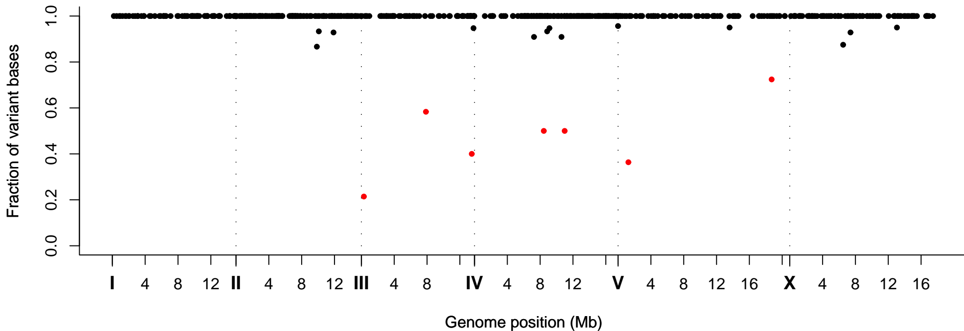
Fraction of Variant Bases at Position, Strain VC40177
