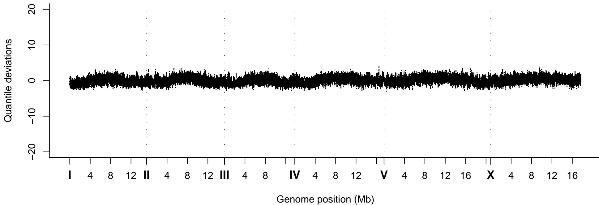
Quantile Deviations, Strain VC40177
