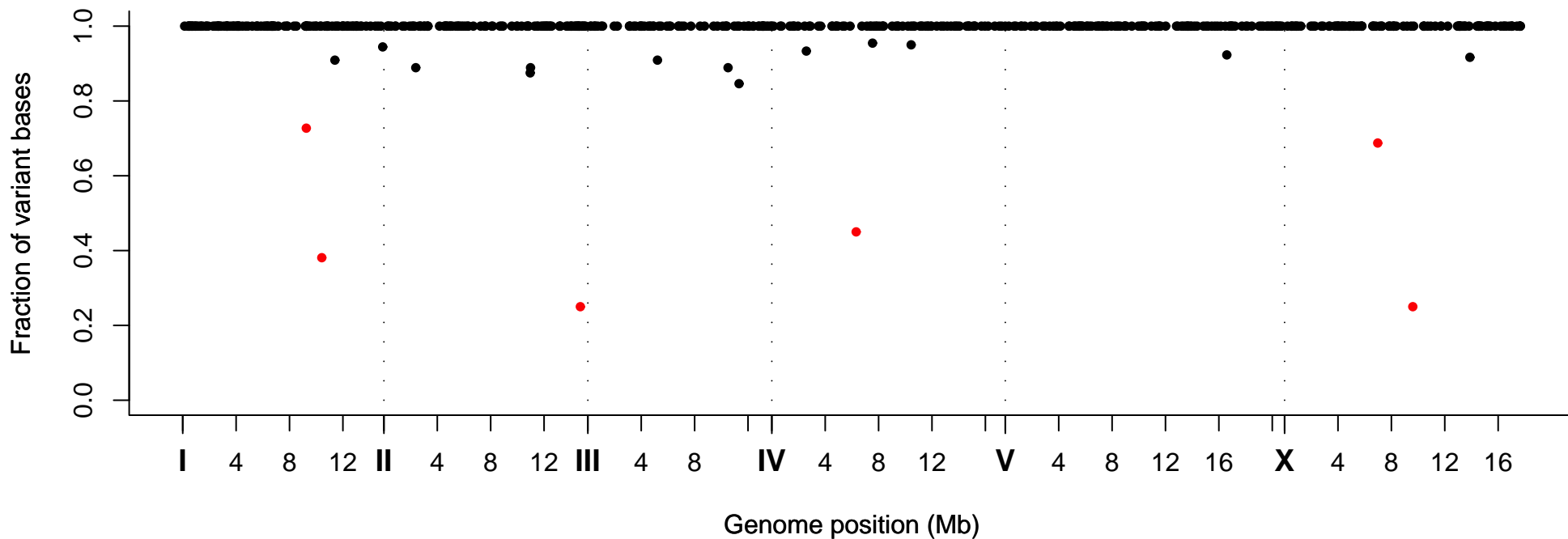
Fraction of Variant Bases at Position, Strain VC40182
