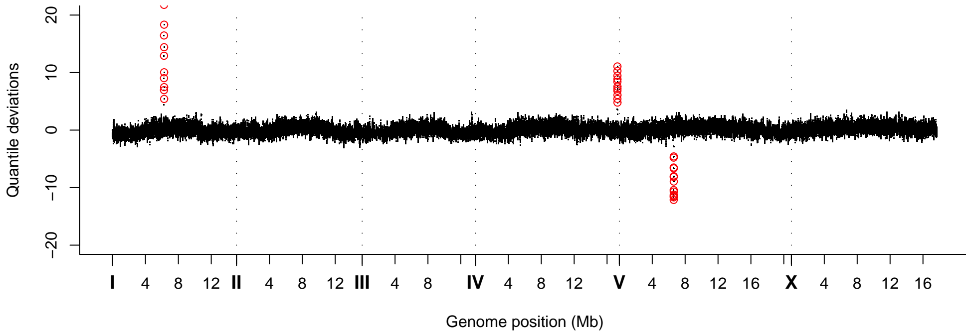
Quantile Deviations, Strain VC40182
