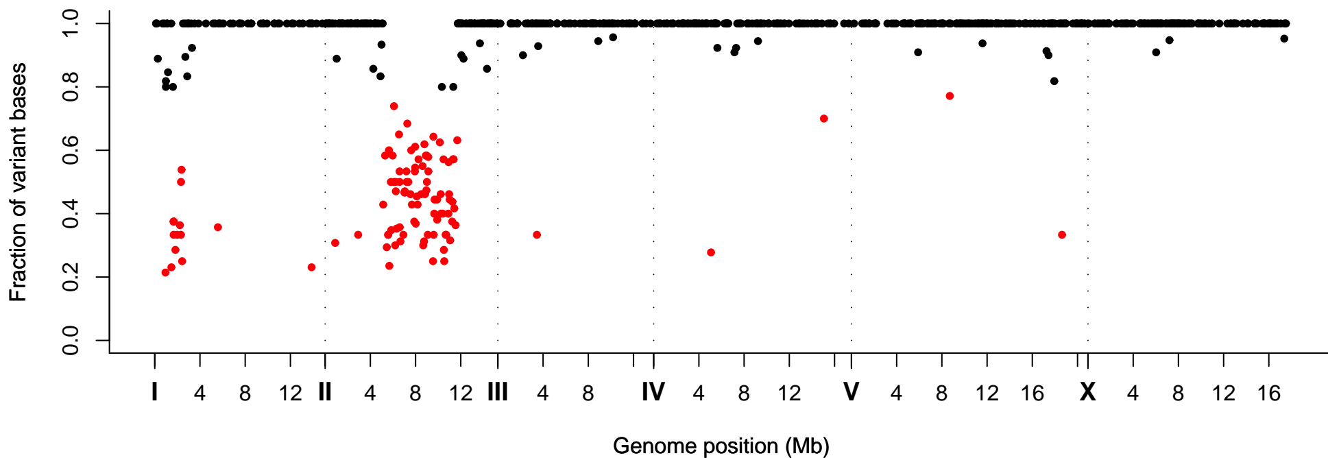
Fraction of Variant Bases at Position, Strain VC40183
