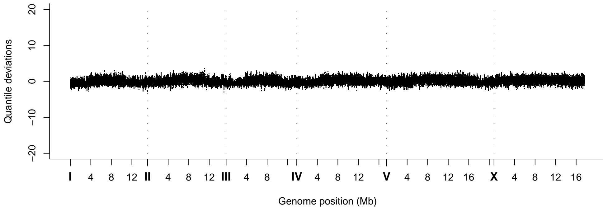
Quantile Deviations, Strain VC40183
