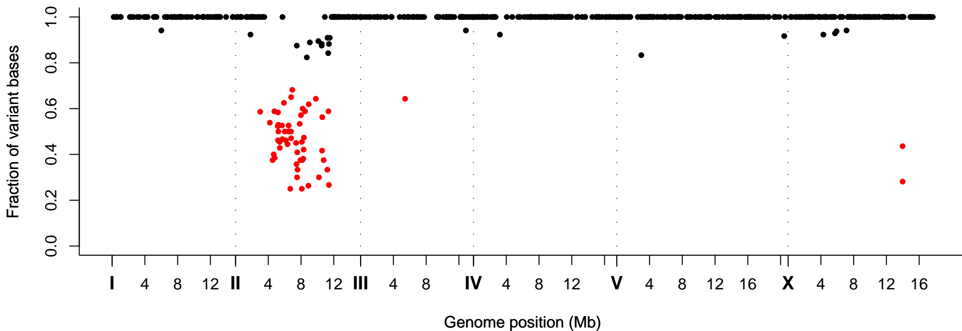
Fraction of Variant Bases at Position, Strain VC40189
