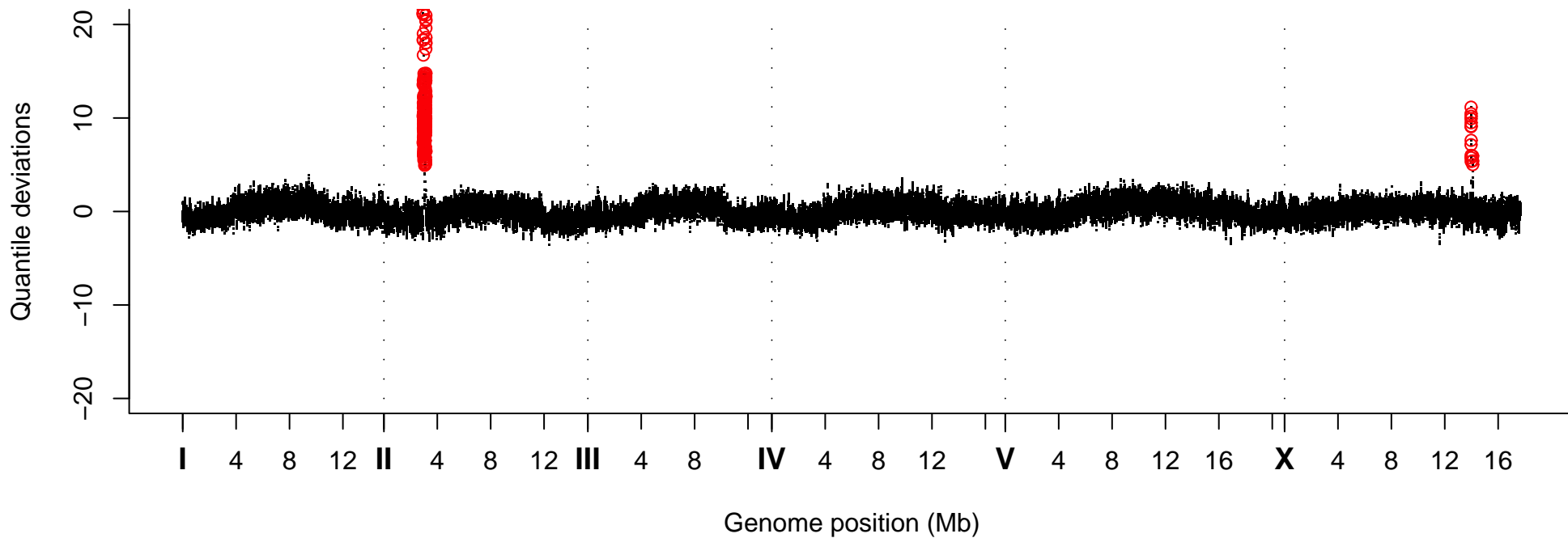
Quantile Deviations, Strain VC40189
