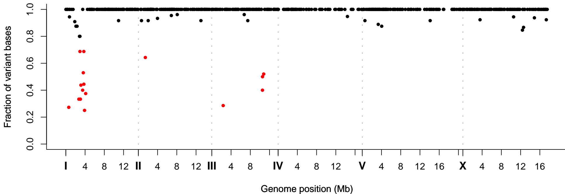
Fraction of Variant Bases at Position, Strain VC40191
