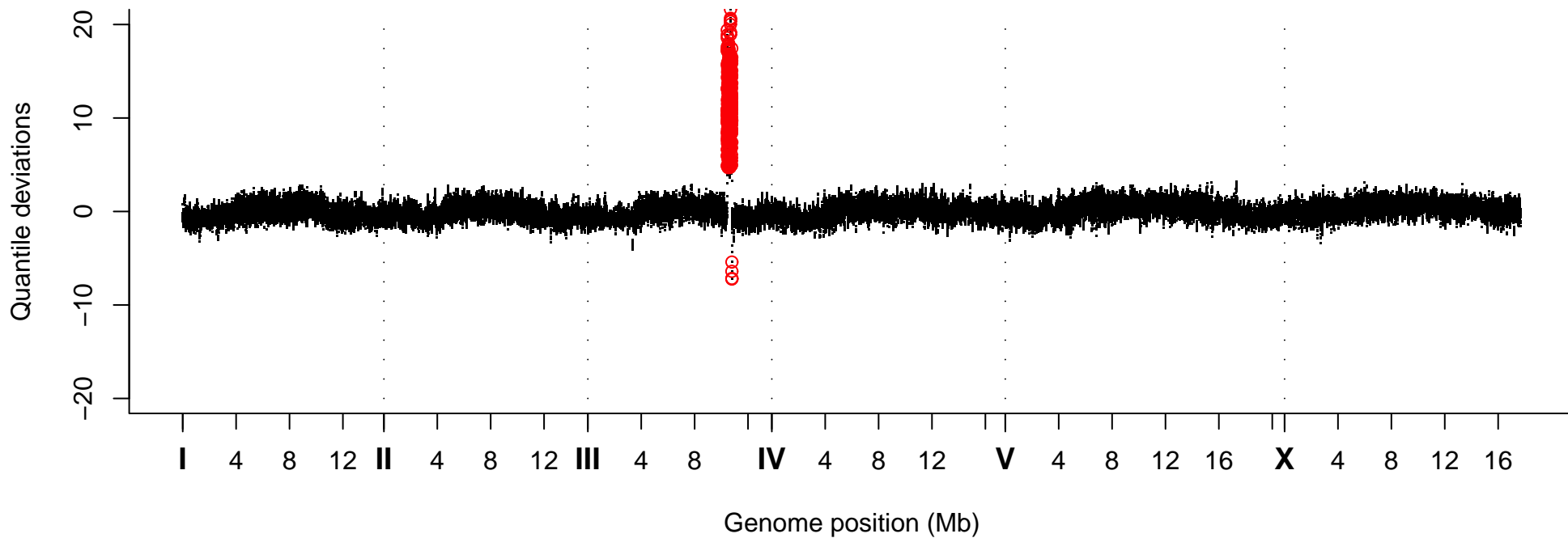
Quantile Deviations, Strain VC40191
