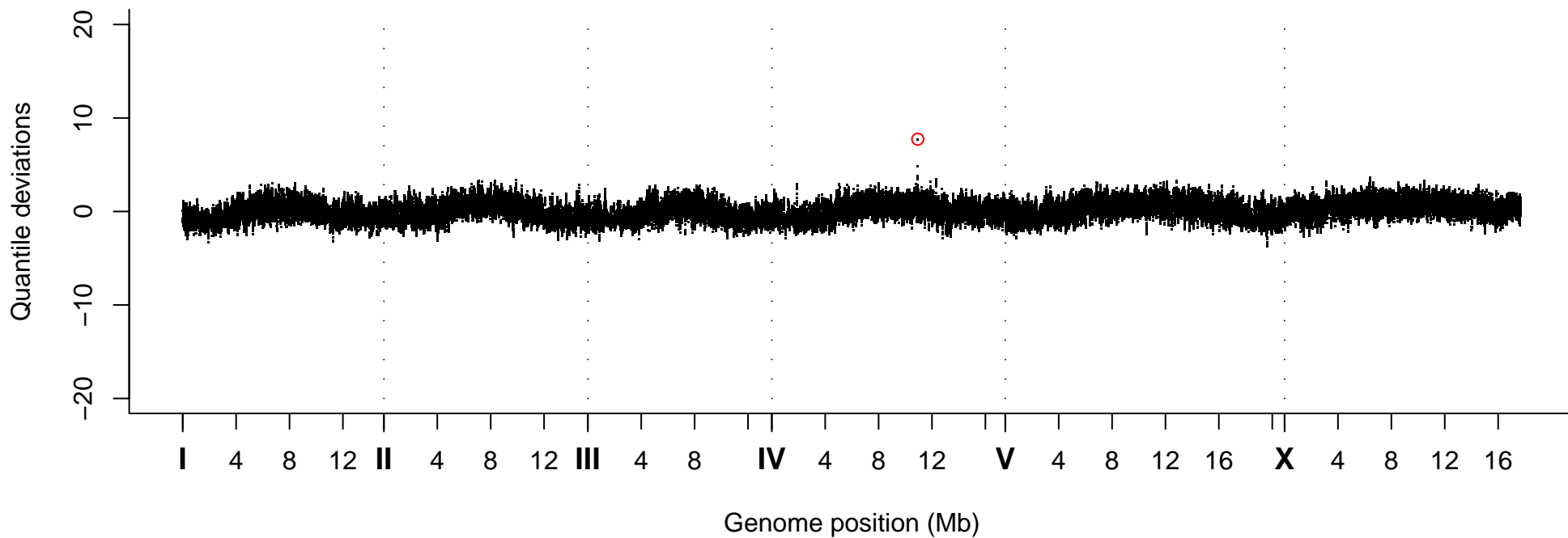
Quantile Deviations, Strain VC40194
