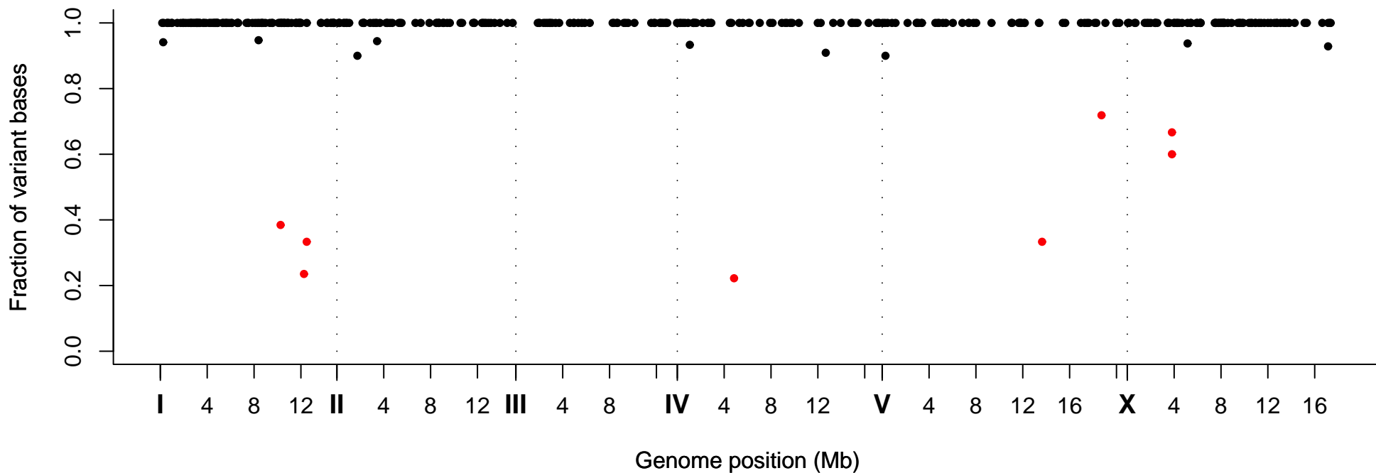
Fraction of Variant Bases at Position, Strain VC40194
