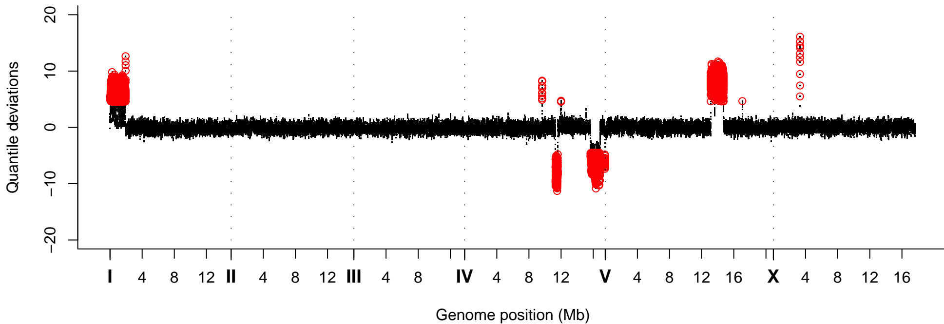
Quantile Deviations, Strain VC40208
