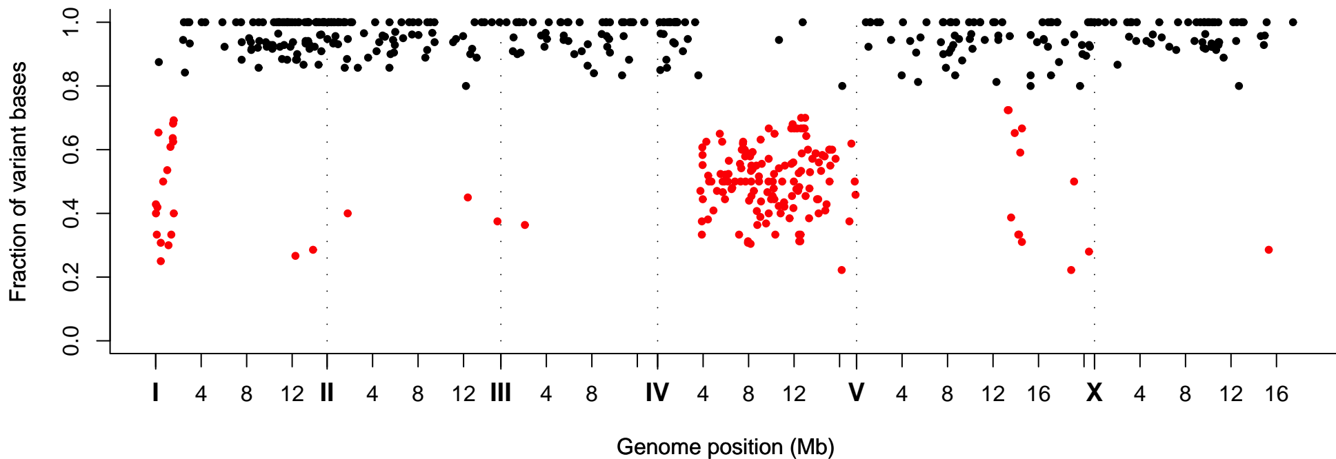
Fraction of Variant Bases at Position, Strain VC40208
