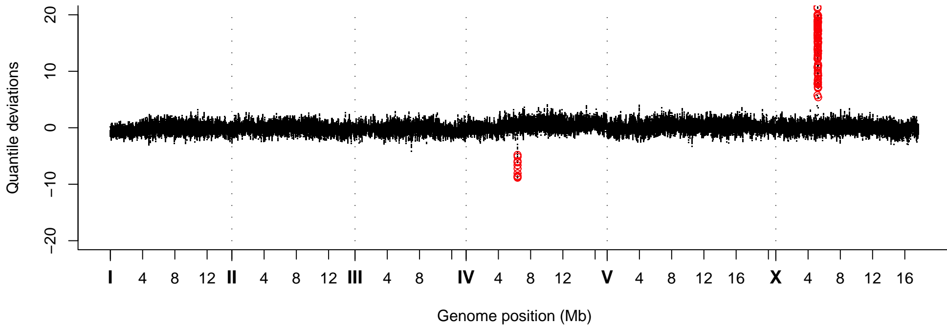
Quantile Deviations, Strain VC40212
