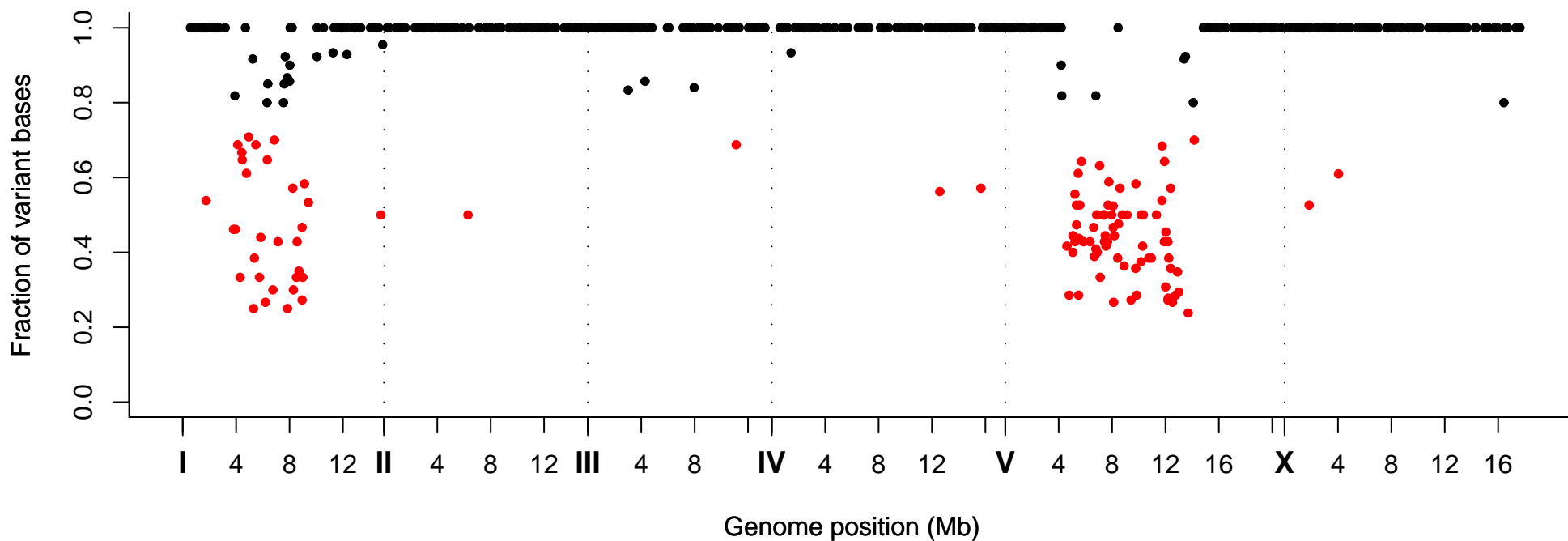
Fraction of Variant Bases at Position, Strain VC40214
