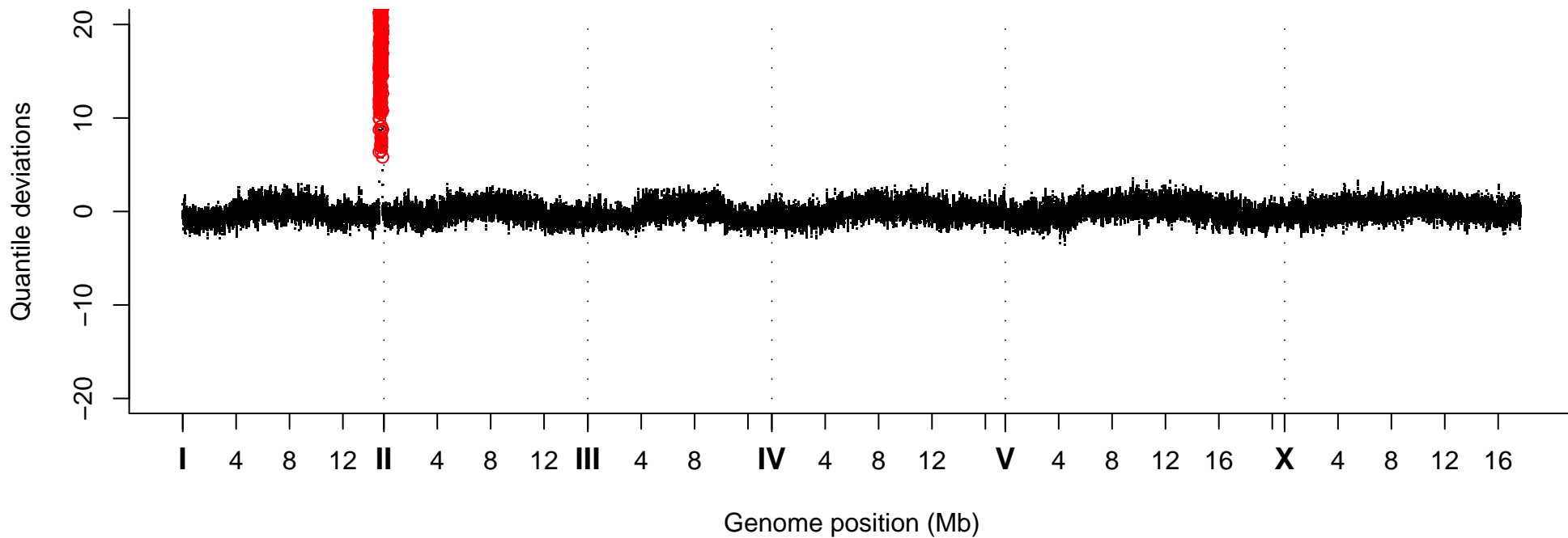
Quantile Deviations, Strain VC40214
