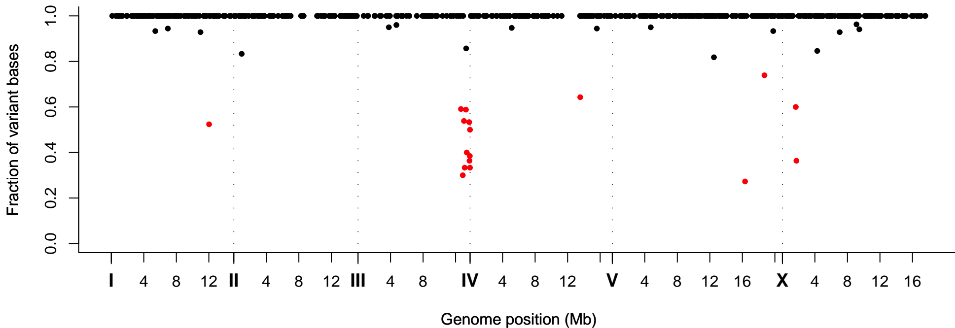
Fraction of Variant Bases at Position, Strain VC40217
