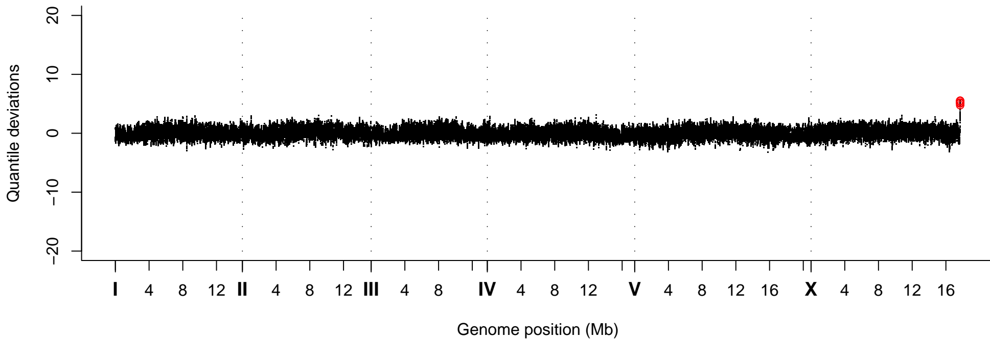
Quantile Deviations, Strain VC40217
