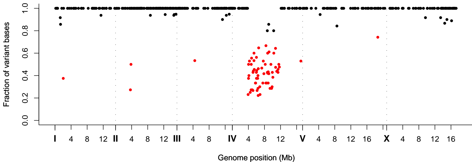
Fraction of Variant Bases at Position, Strain VC40219
