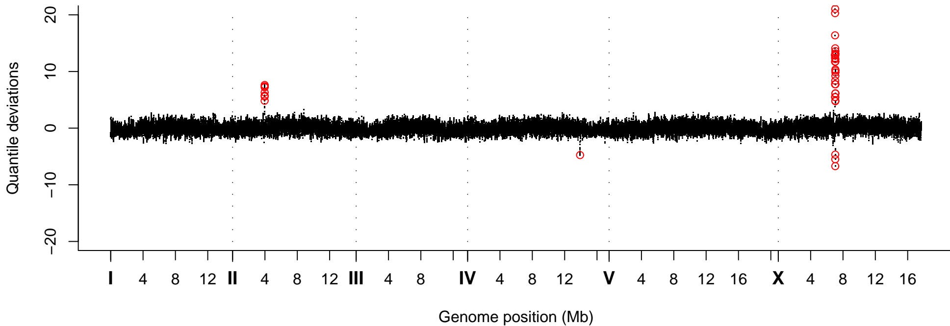
Quantile Deviations, Strain VC40219
