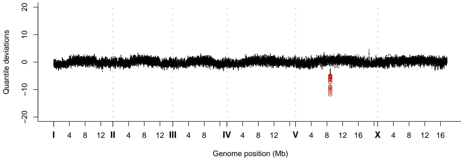
Quantile Deviations, Strain VC40222
