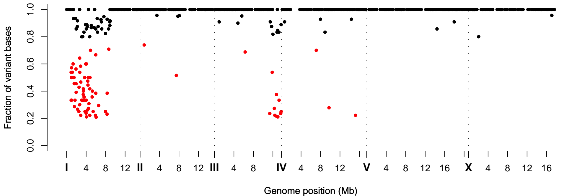
Fraction of Variant Bases at Position, Strain VC40222
