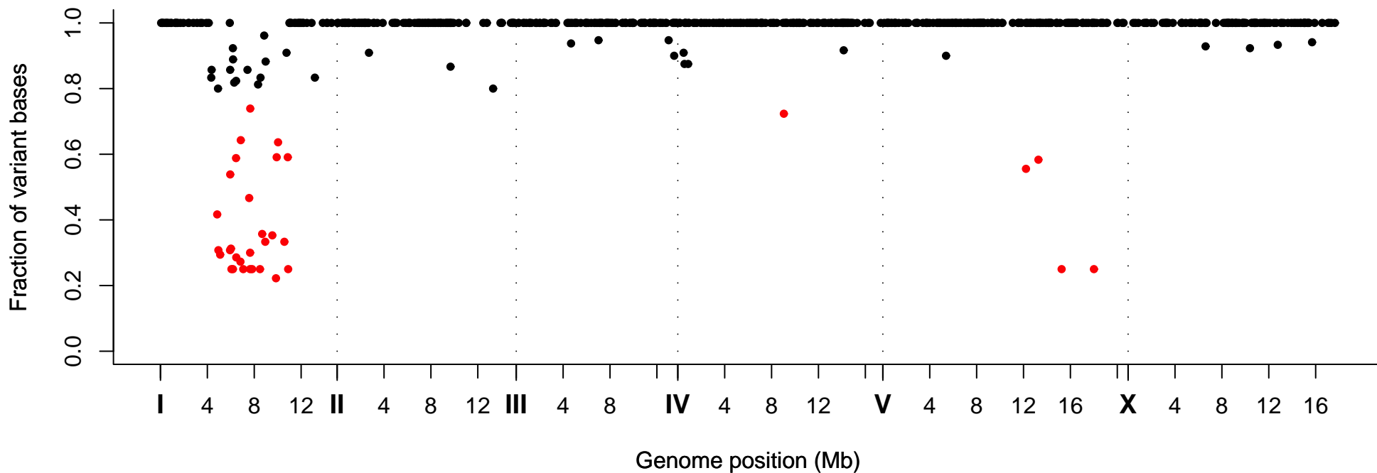
Fraction of Variant Bases at Position, Strain VC40231
