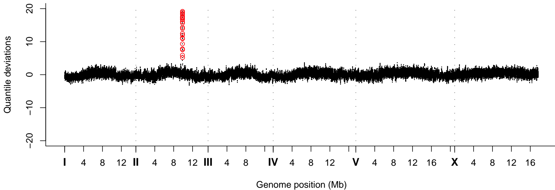
Quantile Deviations, Strain VC40231
