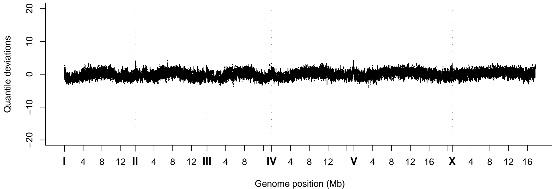
Quantile Deviations, Strain VC40238
