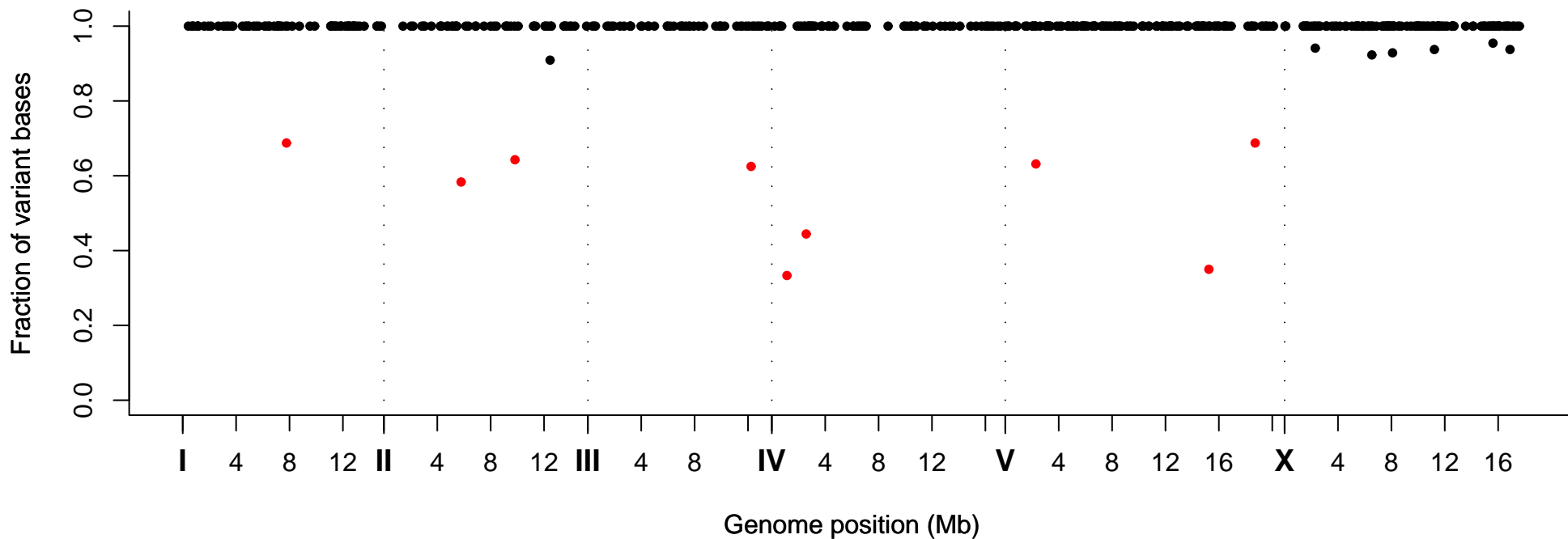
Fraction of Variant Bases at Position, Strain VC40238
