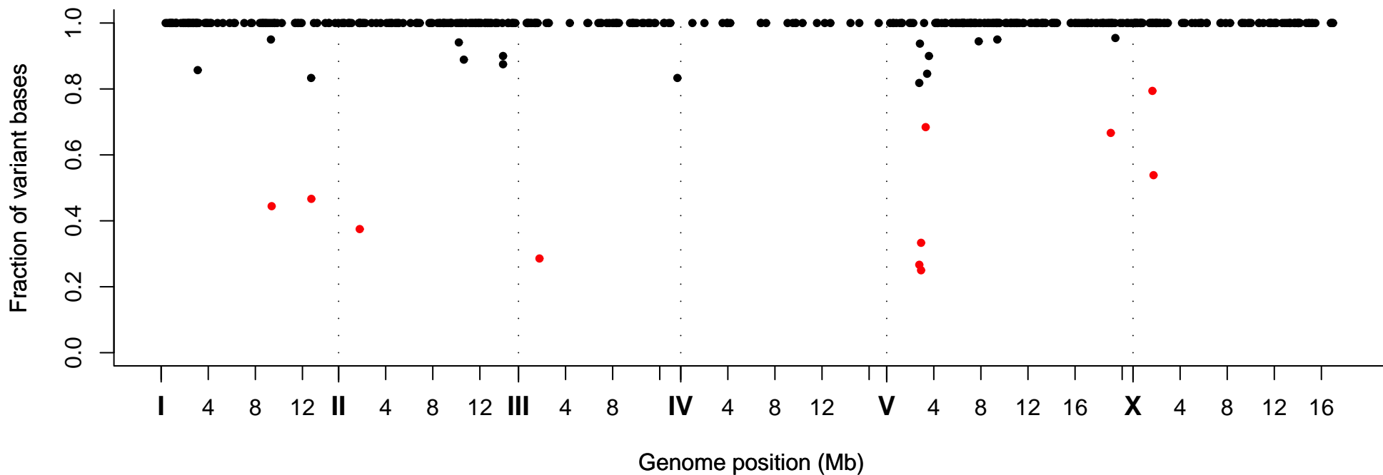
Fraction of Variant Bases at Position, Strain VC40239
