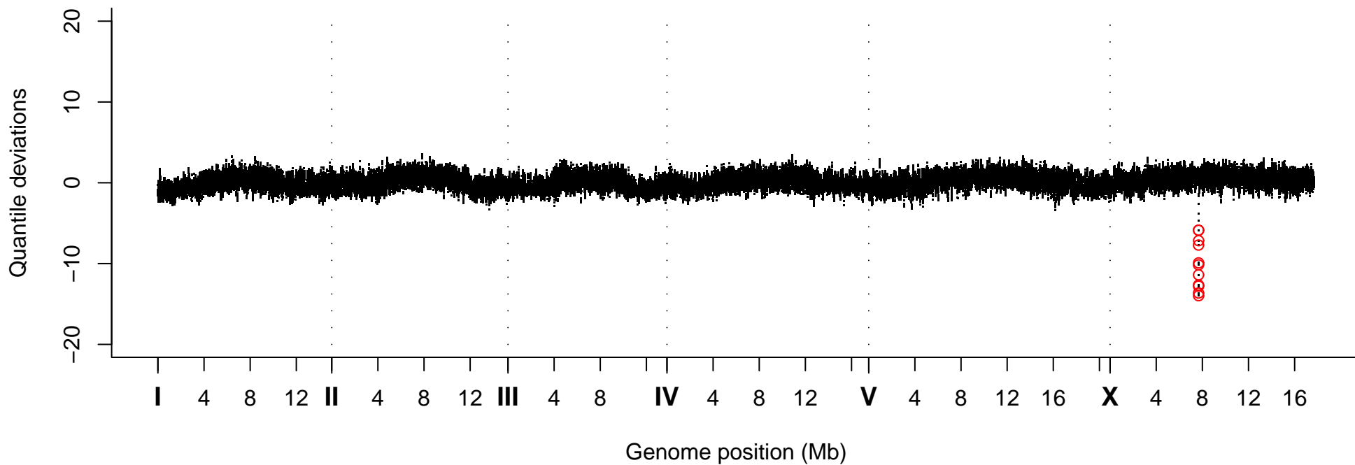
Quantile Deviations, Strain VC40239
