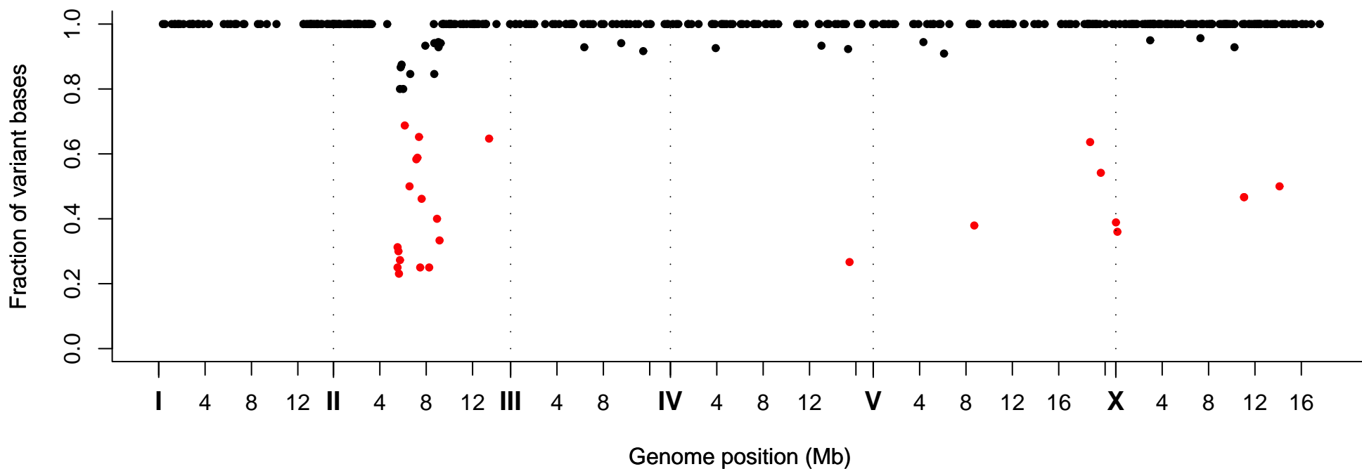
Fraction of Variant Bases at Position, Strain VC40249
