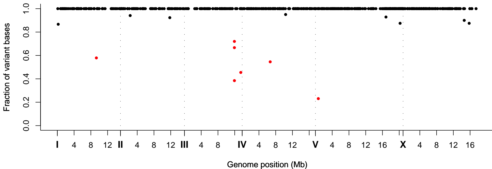
Fraction of Variant Bases at Position, Strain VC40250
