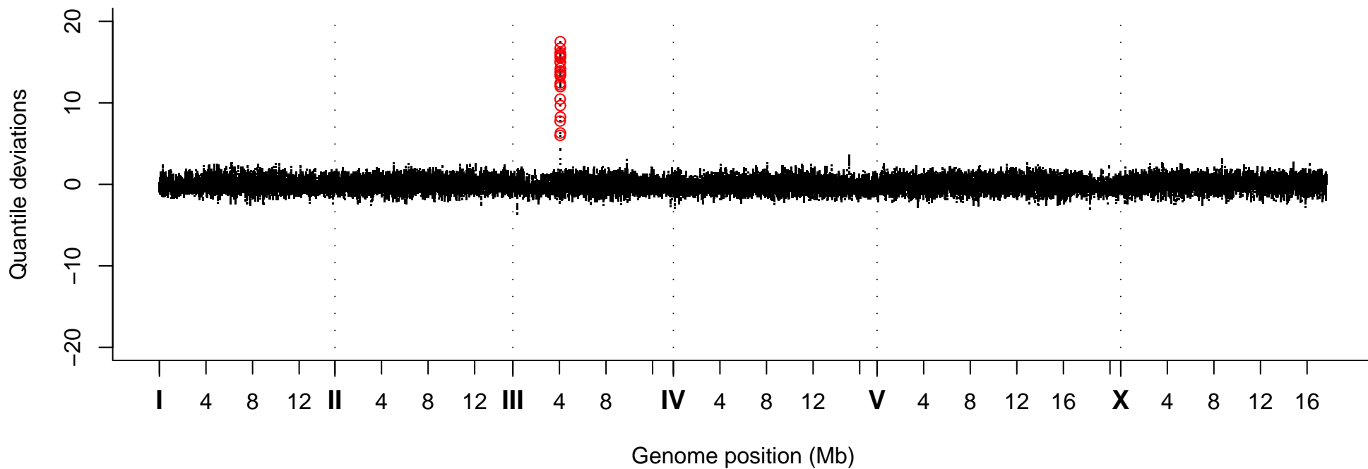
Quantile Deviations, Strain VC40250
