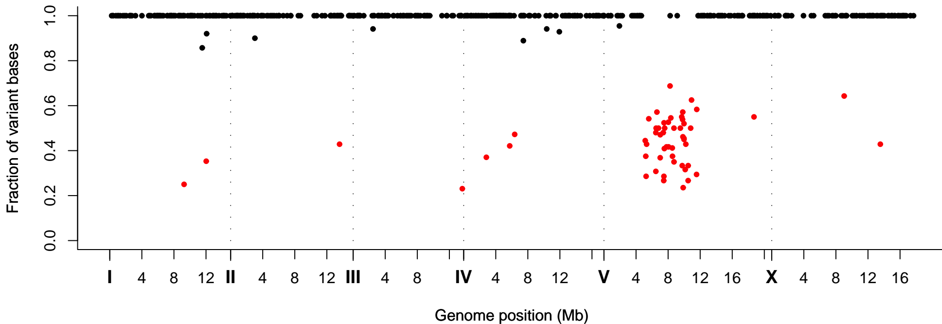
Fraction of Variant Bases at Position, Strain VC40252
