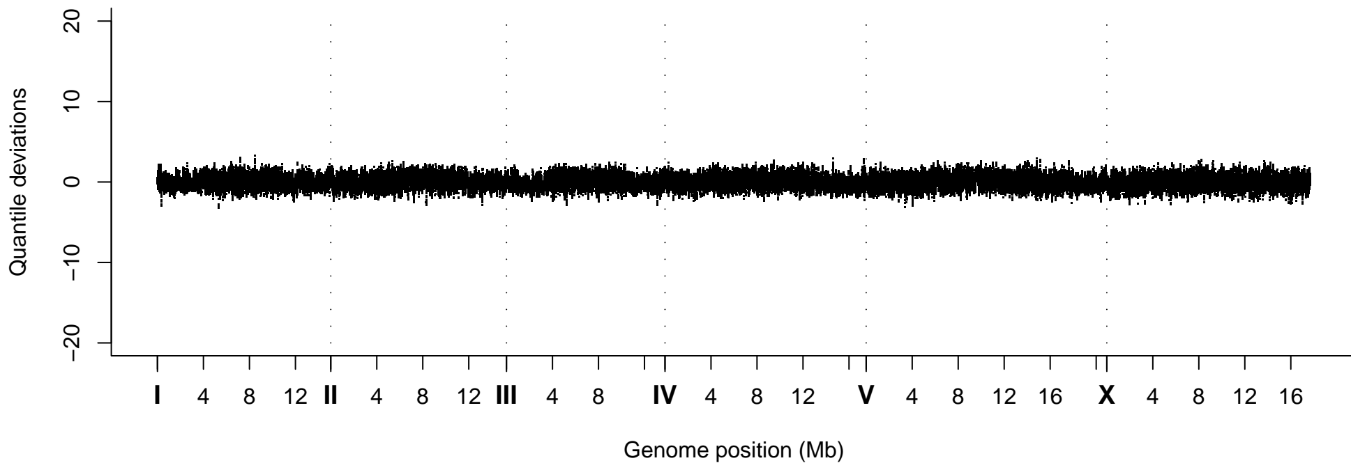
Quantile Deviations, Strain VC40252
